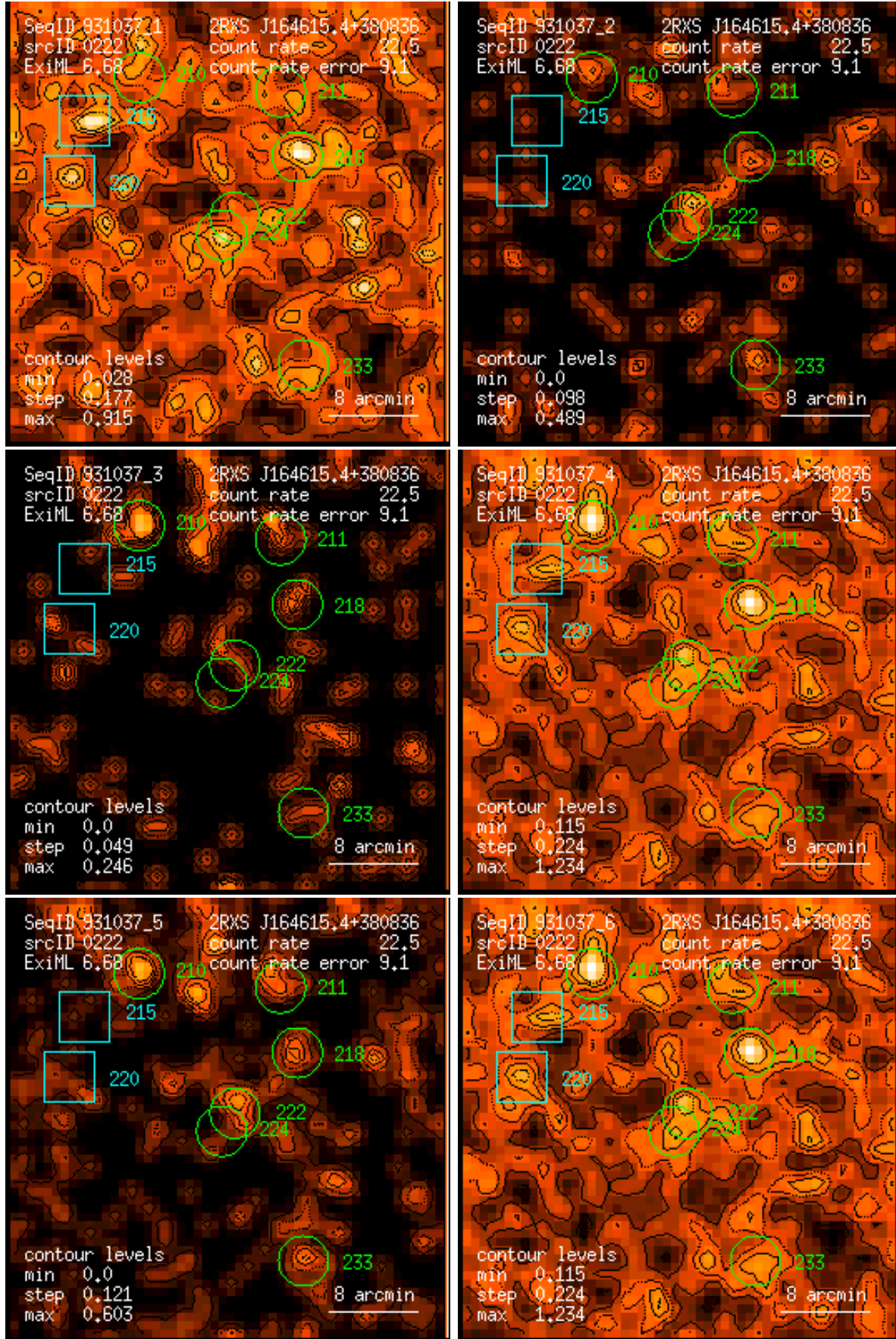
Figure 222: RASS 931037: detection 0222: band rate images, Gaussian filter: (1) PSPC channels 11 – 41, (2) 52 – 90, (3) 91 – 201, (4) 11 – 235, (5) 52 – 201, (6) 11 – 201. Broad band rates in counts/ks. Band rate contour levels in counts/ks/arcmin 2 .
