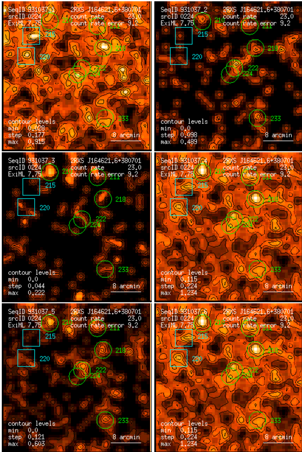
Figure 224: RASS 931037: detection 0224: band rate images, Gaussian filter: (1) PSPC channels 11 – 41, (2) 52 – 90, (3) 91 – 201, (4) 11 – 235, (5) 52 – 201, (6) 11 – 201. Broad band rates in counts/ks. Band rate contour levels in counts/ks/arcmin 2 .
