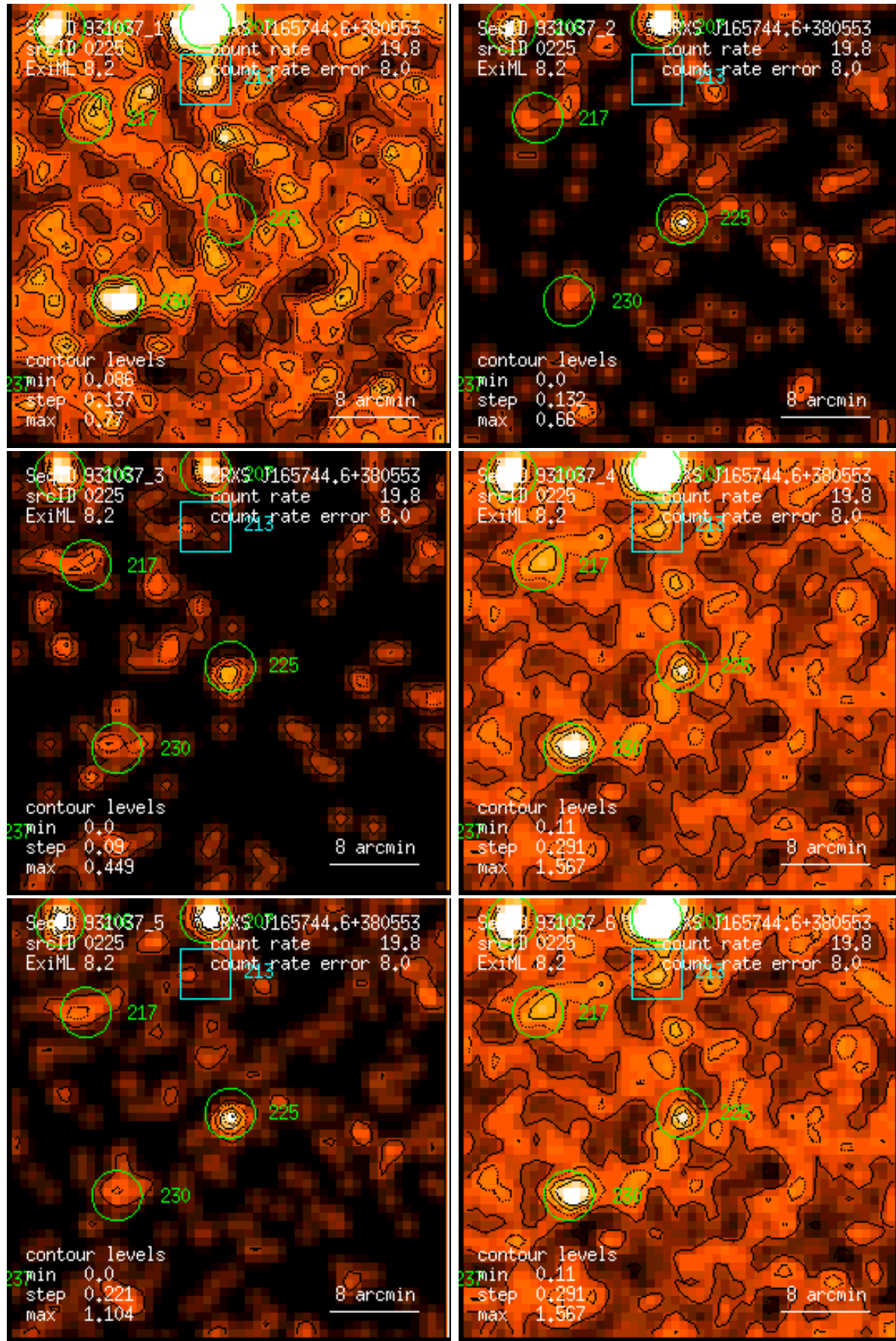
Figure 225: RASS 931037: detection 0225: band rate images, Gaussian filter: (1) PSPC channels 11 – 41, (2) 52 – 90, (3) 91 – 201, (4) 11 – 235, (5) 52 – 201, (6) 11 – 201. Broad band rates in counts/ks. Band rate contour levels in counts/ks/arcmin 2 .
