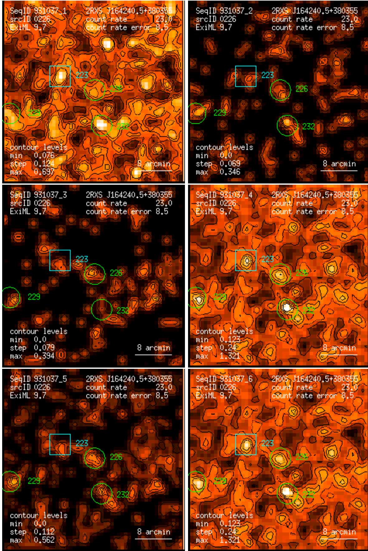
Figure 226: RASS 931037: detection 0226: band rate images, Gaussian filter: (1) PSPC channels 11 – 41, (2) 52 – 90, (3) 91 – 201, (4) 11 – 235, (5) 52 – 201, (6) 11 – 201. Broad band rates in counts/ks. Band rate contour levels in counts/ks/arcmin 2 .
