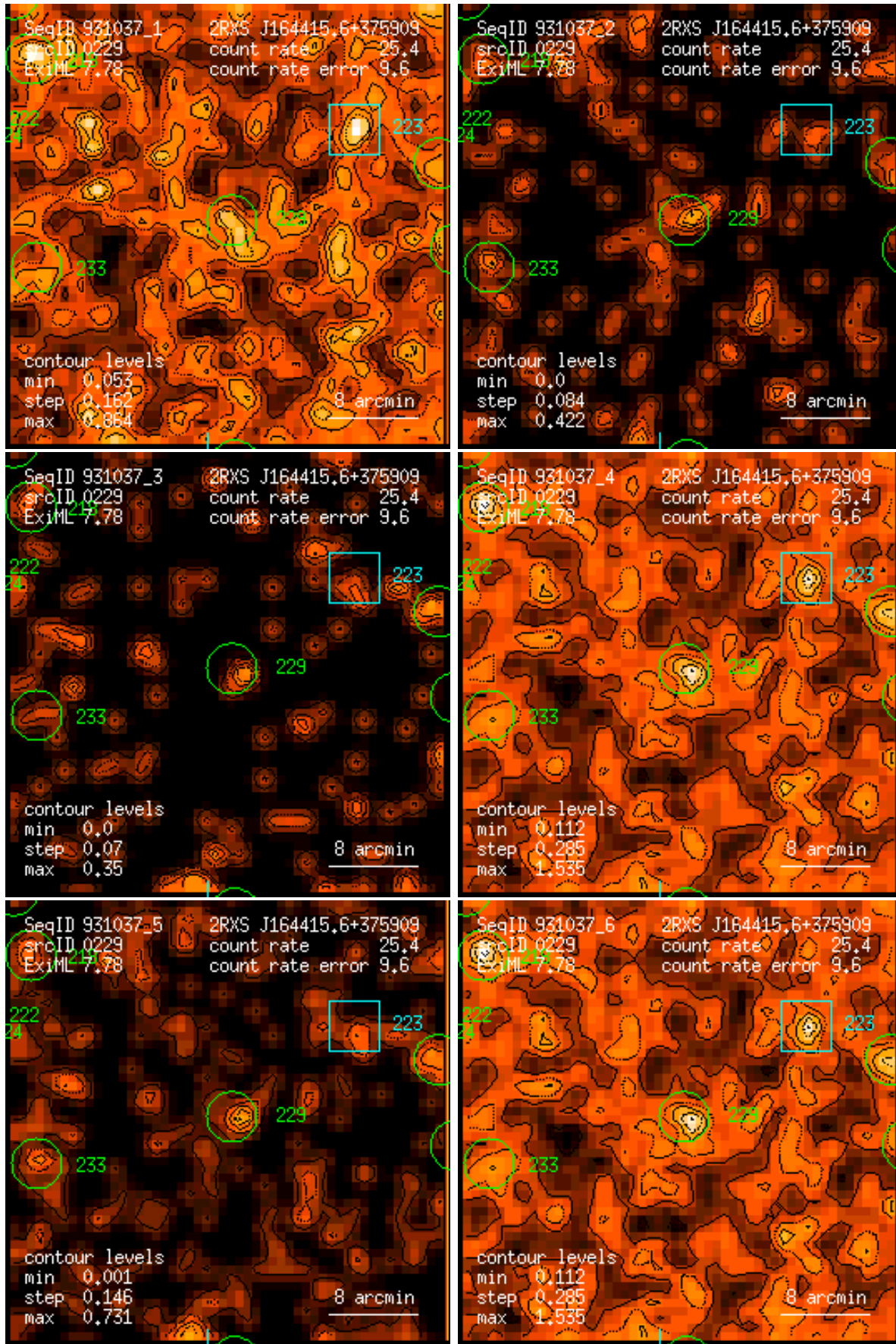
Figure 229: RASS 931037: detection 0229: band rate images, Gaussian filter: (1) PSPC channels 11 – 41, (2) 52 – 90, (3) 91 – 201, (4) 11 – 235, (5) 52 – 201, (6) 11 – 201. Broad band rates in counts/ks. Band rate contour levels in counts/ks/arcmin 2 .
