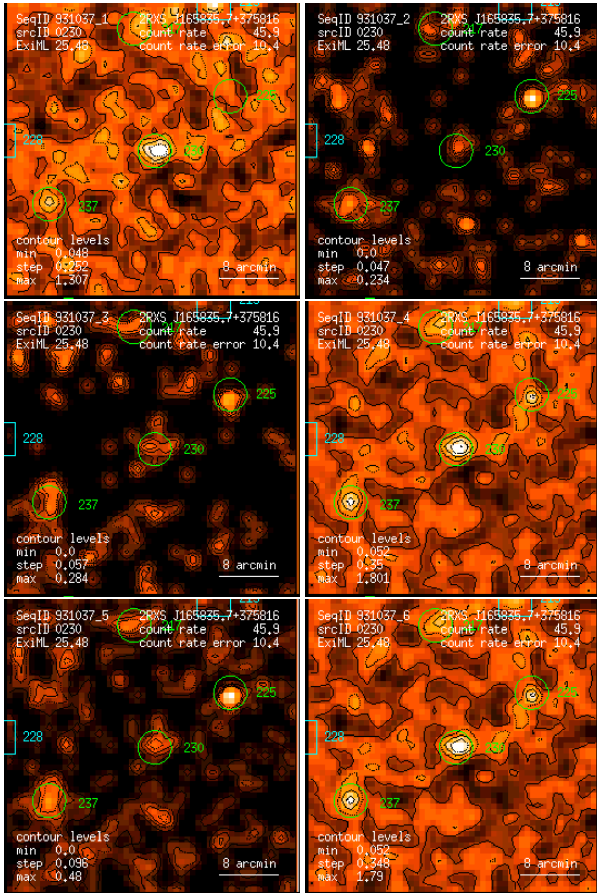
Figure 230: RASS 931037: detection 0230: band rate images, Gaussian filter: (1) PSPC channels 11 – 41, (2) 52 – 90, (3) 91 – 201, (4) 11 – 235, (5) 52 – 201, (6) 11 – 201. Broad band rates in counts/ks. Band rate contour levels in counts/ks/arcmin 2 .
