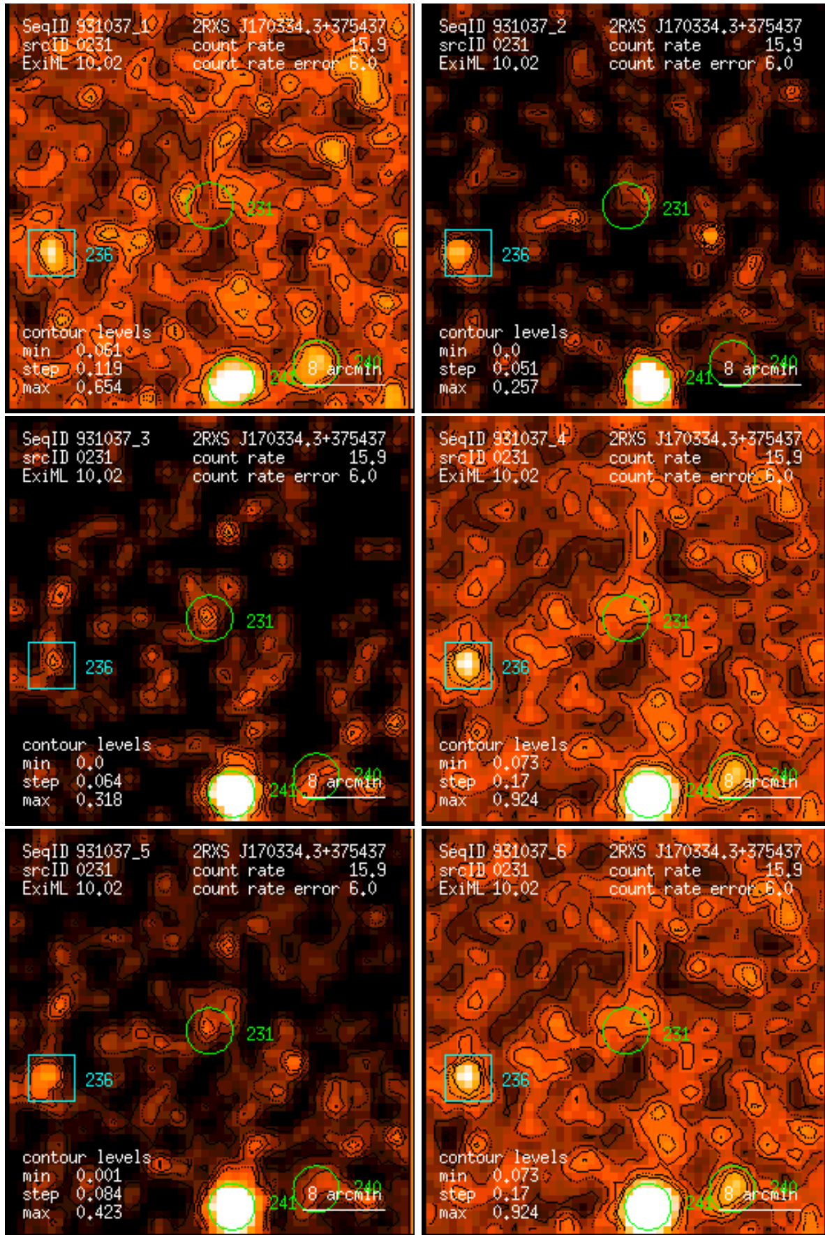
Figure 231: RASS 931037: detection 0231: band rate images, Gaussian filter: (1) PSPC channels 11 – 41, (2) 52 – 90, (3) 91 – 201, (4) 11 – 235, (5) 52 – 201, (6) 11 – 201. Broad band rates in counts/ks. Band rate contour levels in counts/ks/arcmin 2 .
