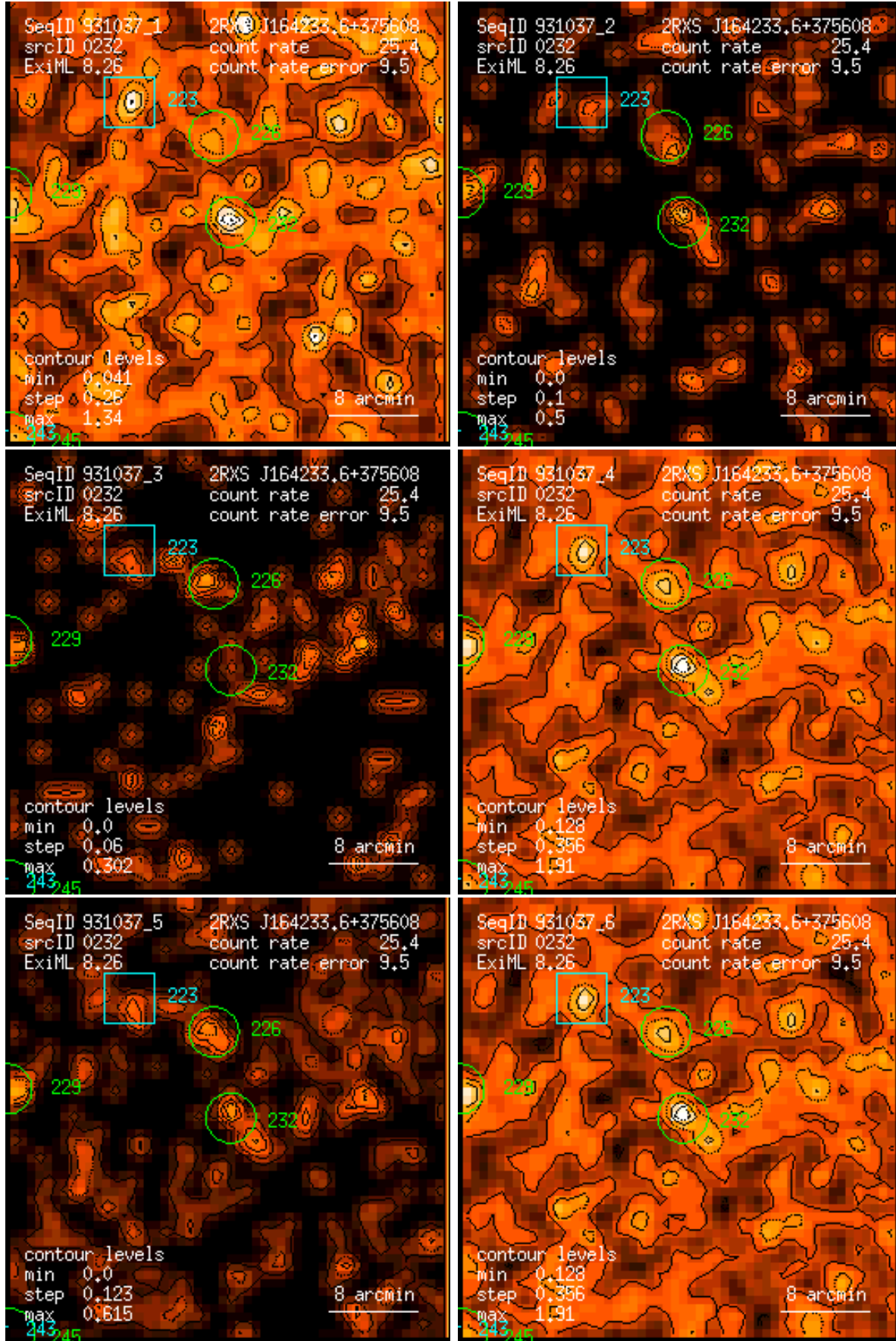
Figure 232: RASS 931037: detection 0232: band rate images, Gaussian filter: (1) PSPC channels 11 – 41, (2) 52 – 90, (3) 91 – 201, (4) 11 – 235, (5) 52 – 201, (6) 11 – 201. Broad band rates in counts/ks. Band rate contour levels in counts/ks/arcmin 2 .
