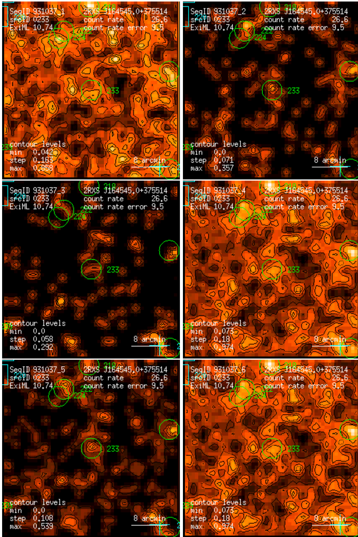
Figure 233: RASS 931037: detection 0233: band rate images, Gaussian filter: (1) PSPC channels 11 – 41, (2) 52 – 90, (3) 91 – 201, (4) 11 – 235, (5) 52 – 201, (6) 11 – 201. Broad band rates in counts/ks. Band rate contour levels in counts/ks/arcmin 2 .
