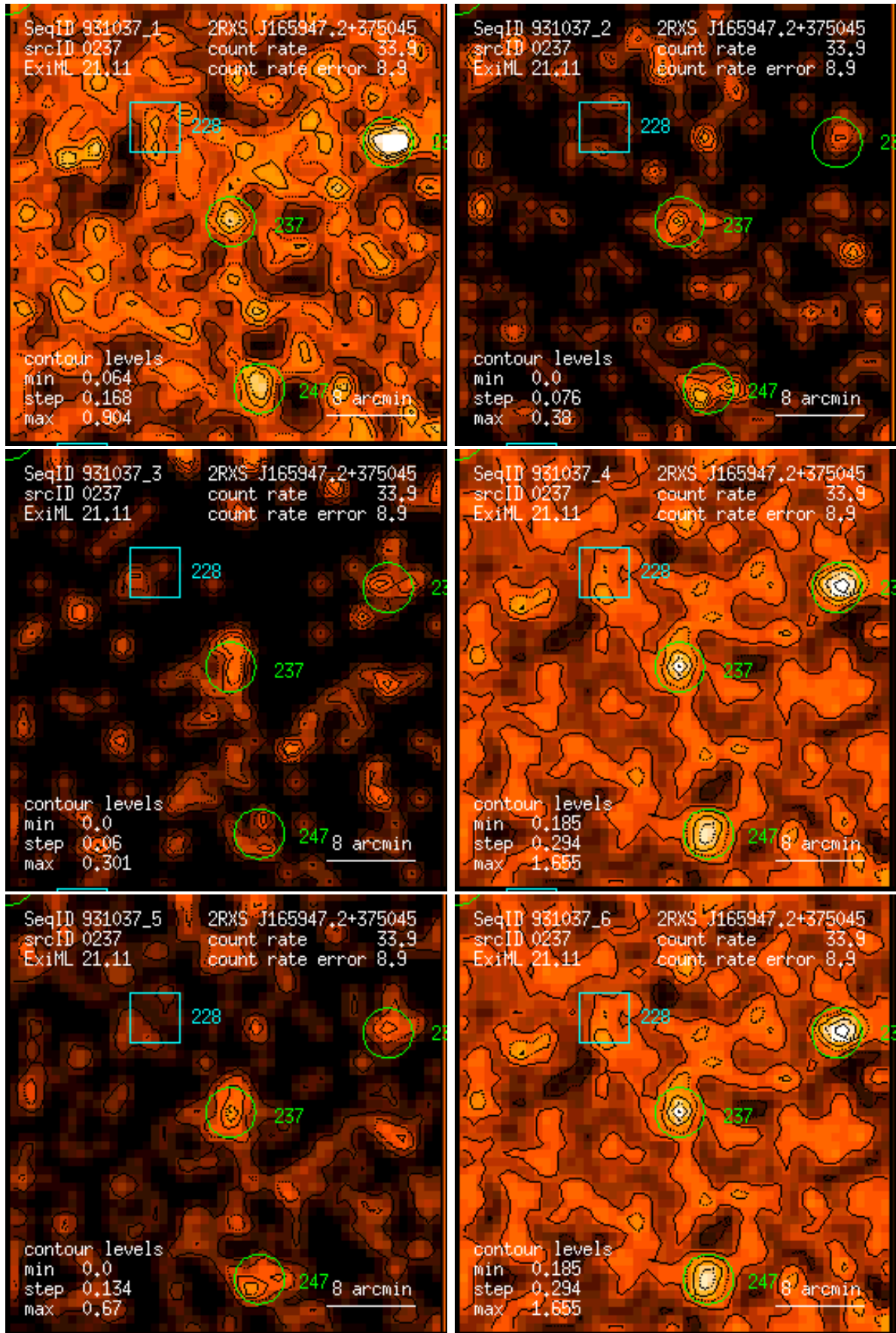
Figure 237: RASS 931037: detection 0237: band rate images, Gaussian filter: (1) PSPC channels 11 – 41, (2) 52 – 90, (3) 91 – 201, (4) 11 – 235, (5) 52 – 201, (6) 11 – 201. Broad band rates in counts/ks. Band rate contour levels in counts/ks/arcmin 2 .
