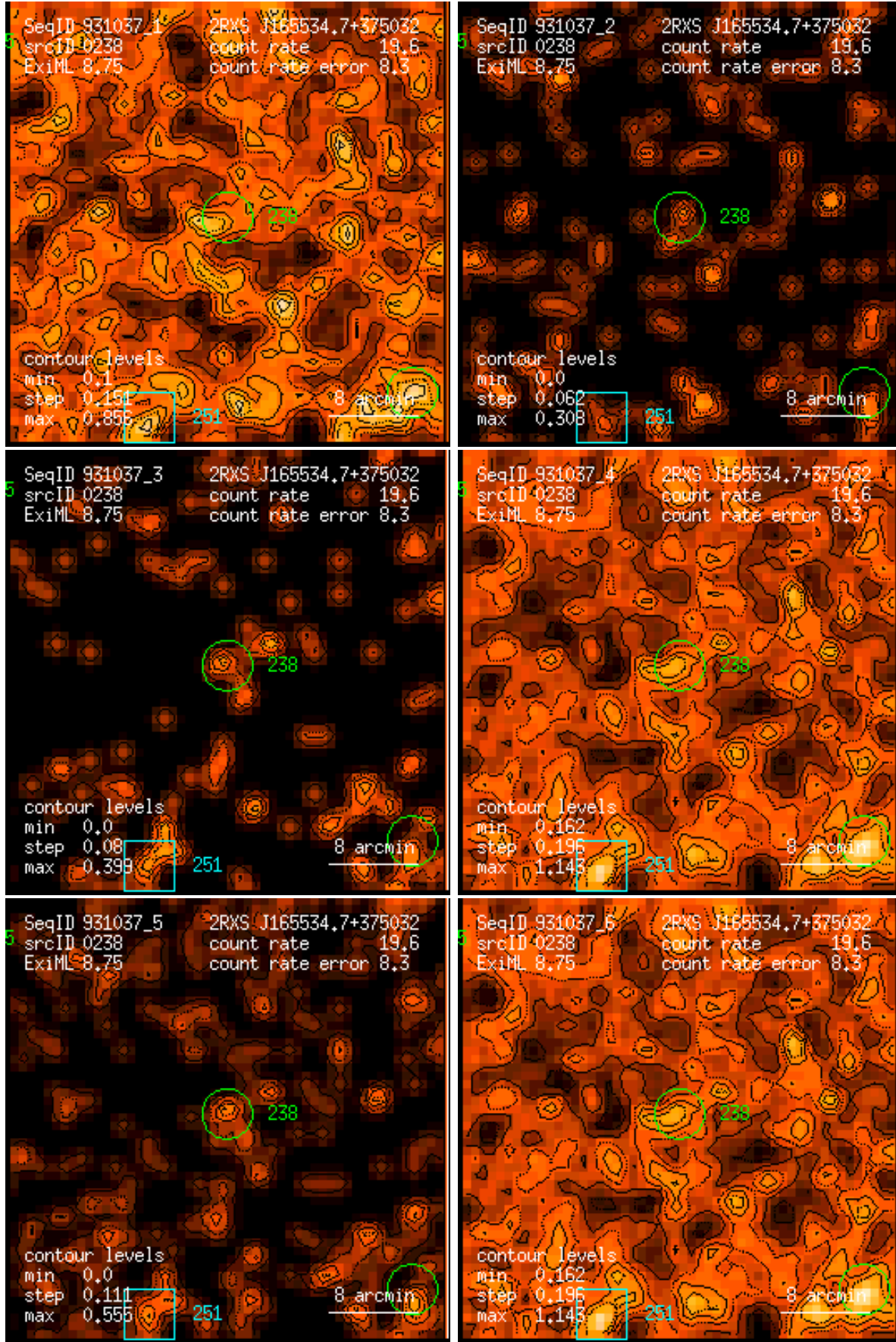
Figure 238: RASS 931037: detection 0238: band rate images, Gaussian filter: (1) PSPC channels 11 – 41, (2) 52 – 90, (3) 91 – 201, (4) 11 – 235, (5) 52 – 201, (6) 11 – 201. Broad band rates in counts/ks. Band rate contour levels in counts/ks/arcmin 2 .
