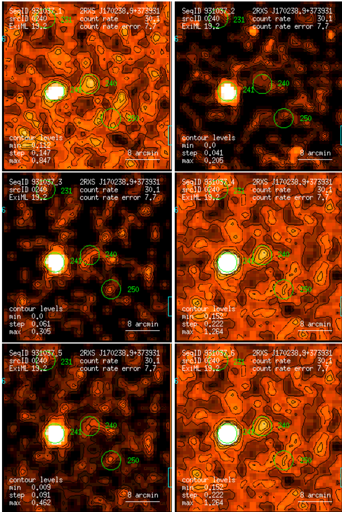
Figure 240: RASS 931037: detection 0240: band rate images, Gaussian filter: (1) PSPC channels 11 – 41, (2) 52 – 90, (3) 91 – 201, (4) 11 – 235, (5) 52 – 201, (6) 11 – 201. Broad band rates in counts/ks. Band rate contour levels in counts/ks/arcmin 2 .
