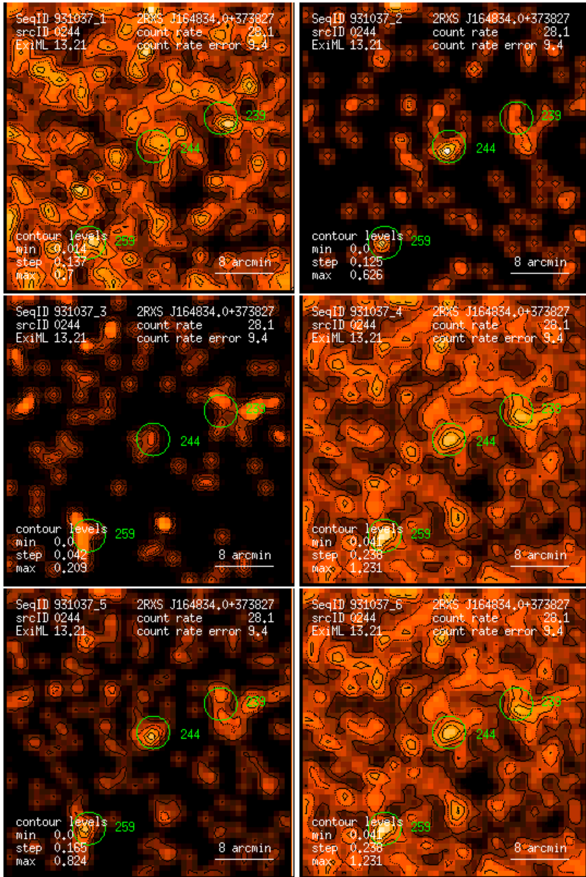
Figure 244: RASS 931037: detection 0244: band rate images, Gaussian filter: (1) PSPC channels 11 – 41, (2) 52 – 90, (3) 91 – 201, (4) 11 – 235, (5) 52 – 201, (6) 11 – 201. Broad band rates in counts/ks. Band rate contour levels in counts/ks/arcmin 2 .
