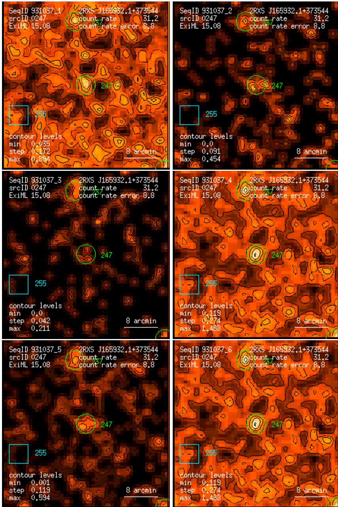
Figure 247: RASS 931037: detection 0247: band rate images, Gaussian filter: (1) PSPC channels 11 – 41, (2) 52 – 90, (3) 91 – 201, (4) 11 – 235, (5) 52 – 201, (6) 11 – 201. Broad band rates in counts/ks. Band rate contour levels in counts/ks/arcmin 2 .
