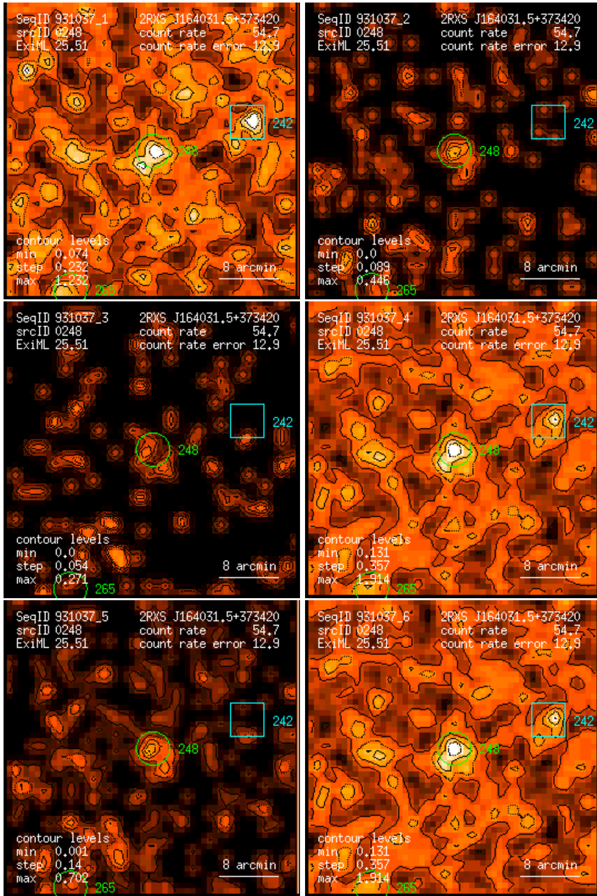
Figure 248: RASS 931037: detection 0248: band rate images, Gaussian filter: (1) PSPC channels 11 – 41, (2) 52 – 90, (3) 91 – 201, (4) 11 – 235, (5) 52 – 201, (6) 11 – 201. Broad band rates in counts/ks. Band rate contour levels in counts/ks/arcmin 2 .
