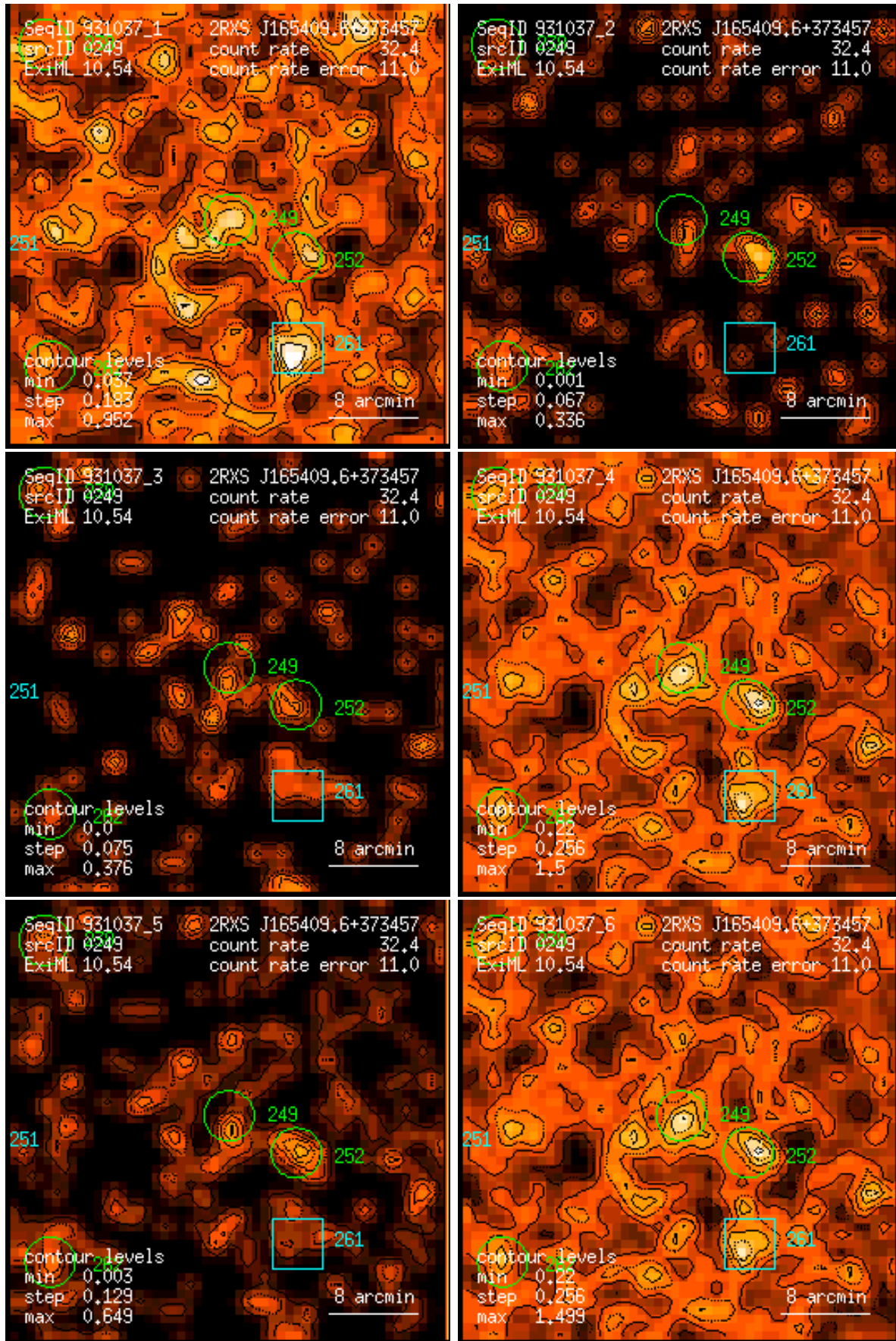
Figure 249: RASS 931037: detection 0249: band rate images, Gaussian filter: (1) PSPC channels 11 – 41, (2) 52 – 90, (3) 91 – 201, (4) 11 – 235, (5) 52 – 201, (6) 11 – 201. Broad band rates in counts/ks. Band rate contour levels in counts/ks/arcmin 2 .
