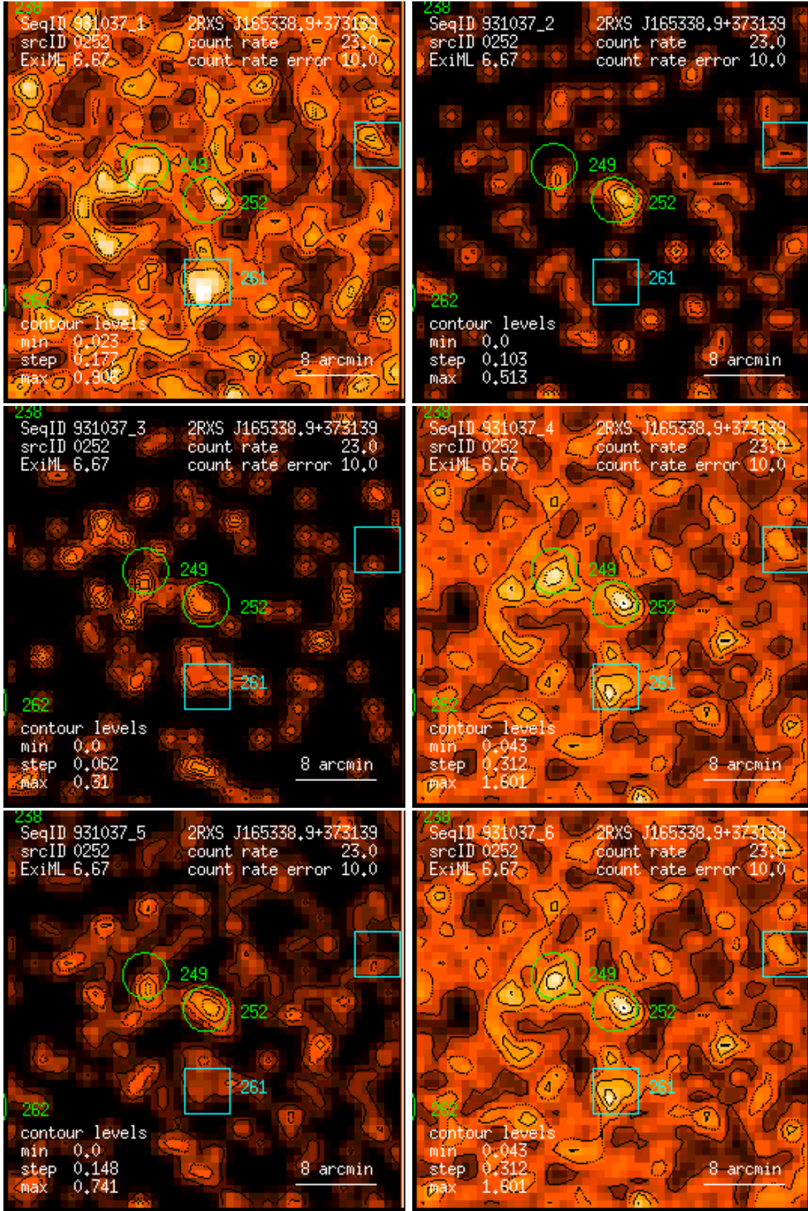
Figure 252: RASS 931037: detection 0252: band rate images, Gaussian filter: (1) PSPC channels 11 – 41, (2) 52 – 90, (3) 91 – 201, (4) 11 – 235, (5) 52 – 201, (6) 11 – 201. Broad band rates in counts/ks. Band rate contour levels in counts/ks/arcmin 2 .
