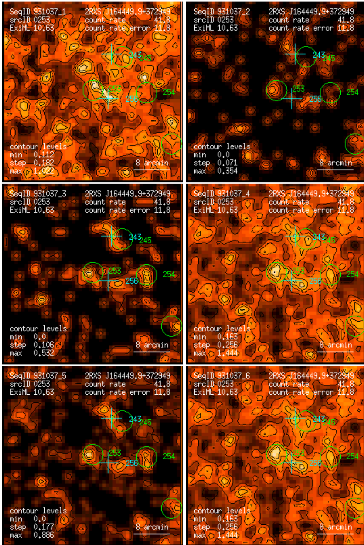
Figure 253: RASS 931037: detection 0253: band rate images, Gaussian filter: (1) PSPC channels 11 – 41, (2) 52 – 90, (3) 91 – 201, (4) 11 – 235, (5) 52 – 201, (6) 11 – 201. Broad band rates in counts/ks. Band rate contour levels in counts/ks/arcmin 2 .
