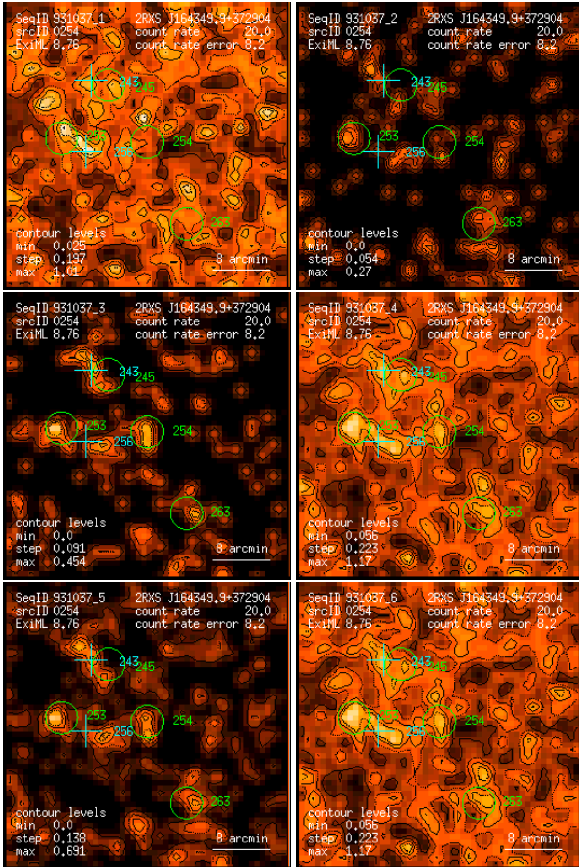
Figure 254: RASS 931037: detection 0254: band rate images, Gaussian filter: (1) PSPC channels 11 – 41, (2) 52 – 90, (3) 91 – 201, (4) 11 – 235, (5) 52 – 201, (6) 11 – 201. Broad band rates in counts/ks. Band rate contour levels in counts/ks/arcmin 2 .
