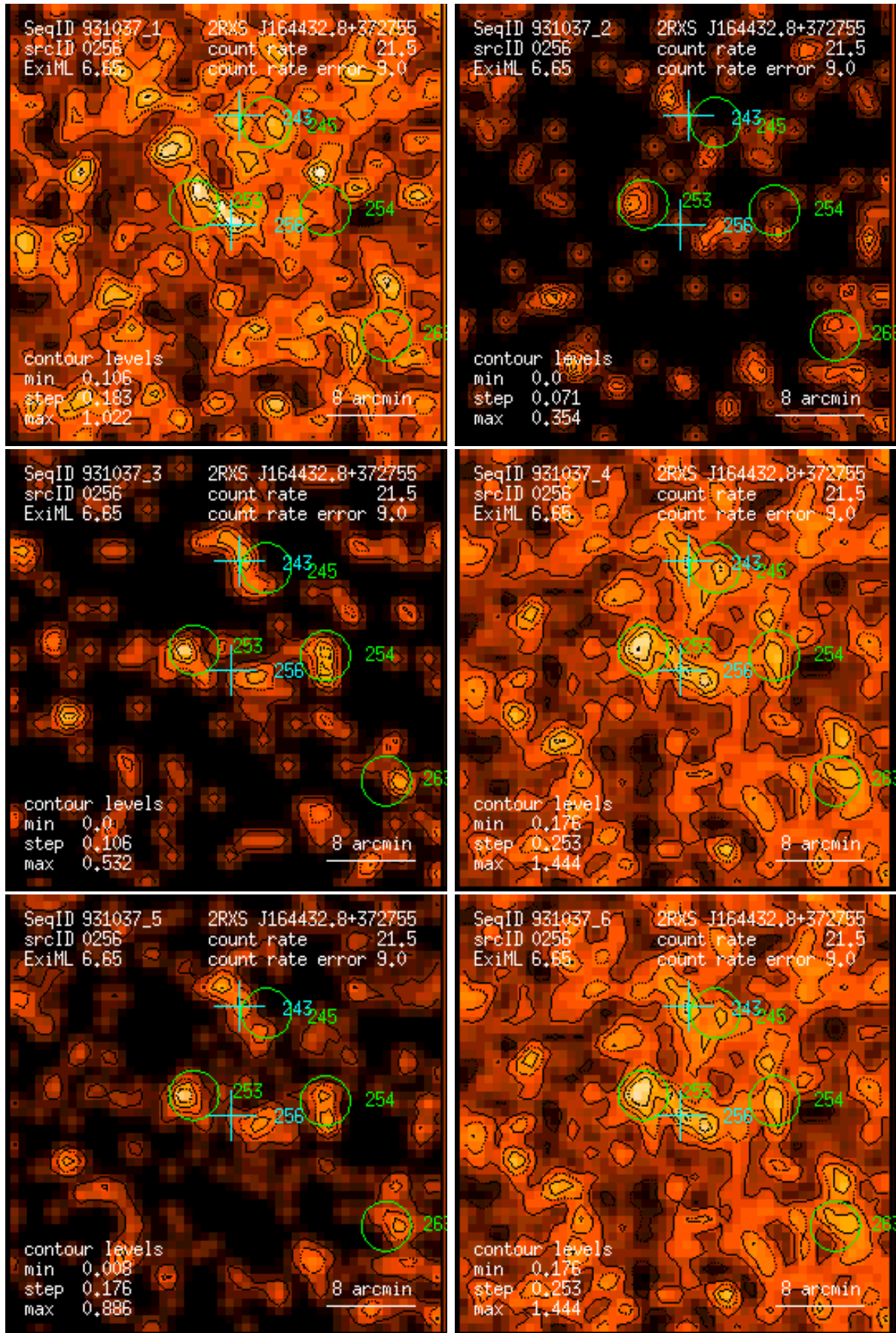
Figure 256: RASS 931037: detection 0256: band rate images, Gaussian filter: (1) PSPC channels 11 – 41, (2) 52 – 90, (3) 91 – 201, (4) 11 – 235, (5) 52 – 201, (6) 11 – 201. Broad band rates in counts/ks. Band rate contour levels in counts/ks/arcmin 2 .
