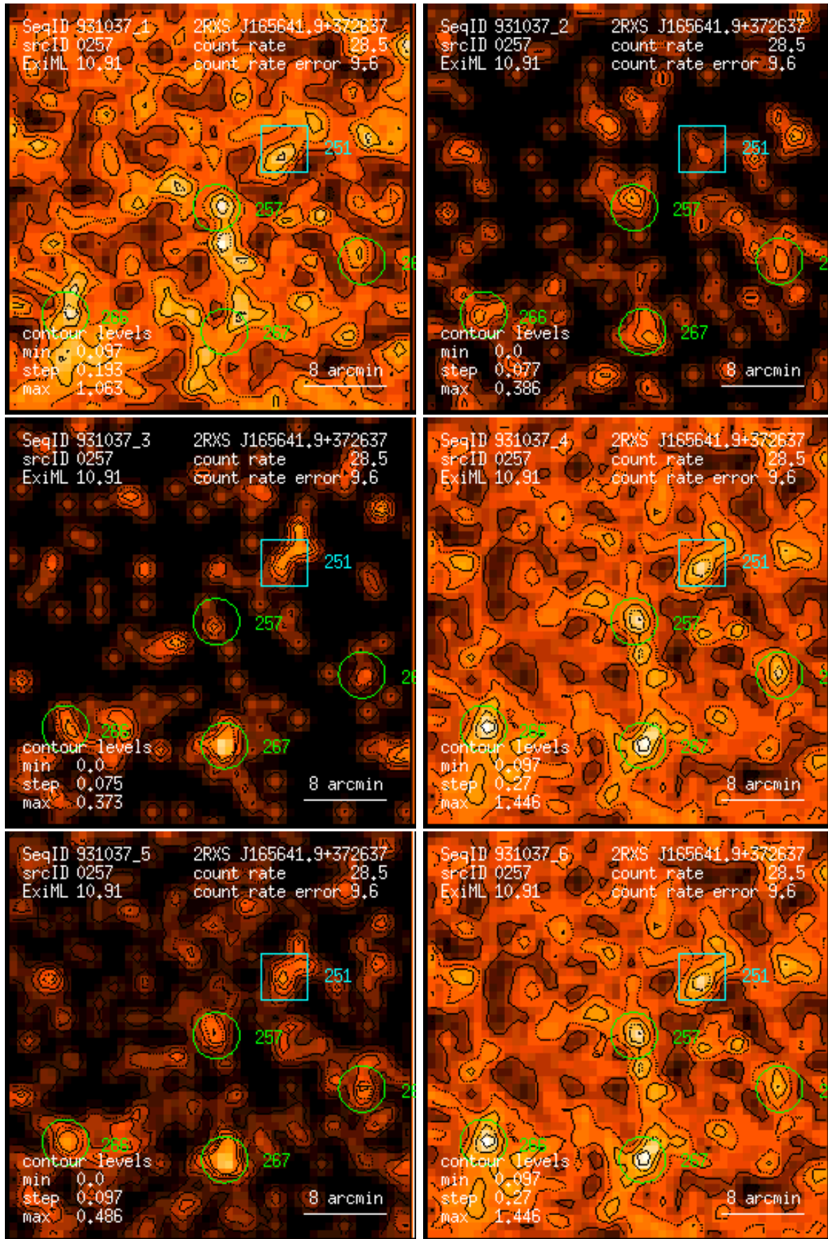
Figure 257: RASS 931037: detection 0257: band rate images, Gaussian filter: (1) PSPC channels 11 – 41, (2) 52 – 90, (3) 91 – 201, (4) 11 – 235, (5) 52 – 201, (6) 11 – 201. Broad band rates in counts/ks. Band rate contour levels in counts/ks/arcmin 2 .
