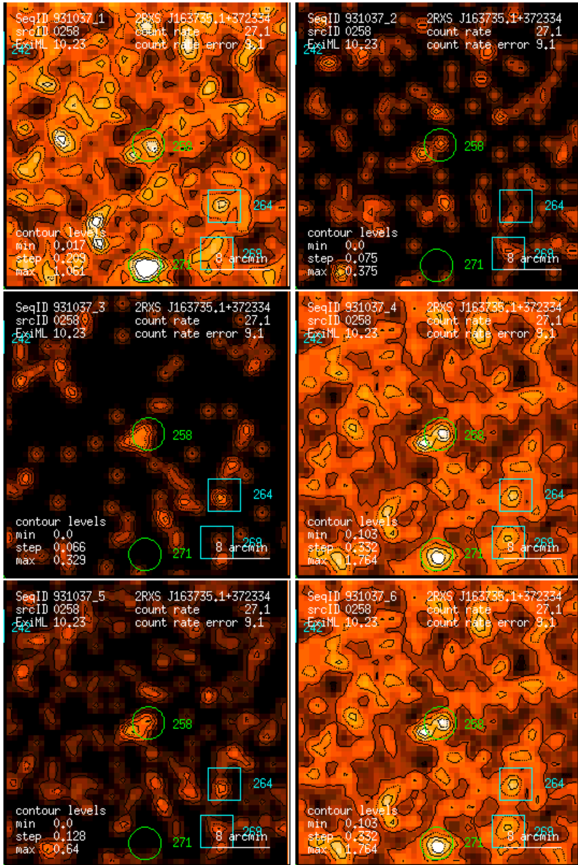
Figure 258: RASS 931037: detection 0258: band rate images, Gaussian filter: (1) PSPC channels 11 – 41, (2) 52 – 90, (3) 91 – 201, (4) 11 – 235, (5) 52 – 201, (6) 11 – 201. Broad band rates in counts/ks. Band rate contour levels in counts/ks/arcmin 2 .
