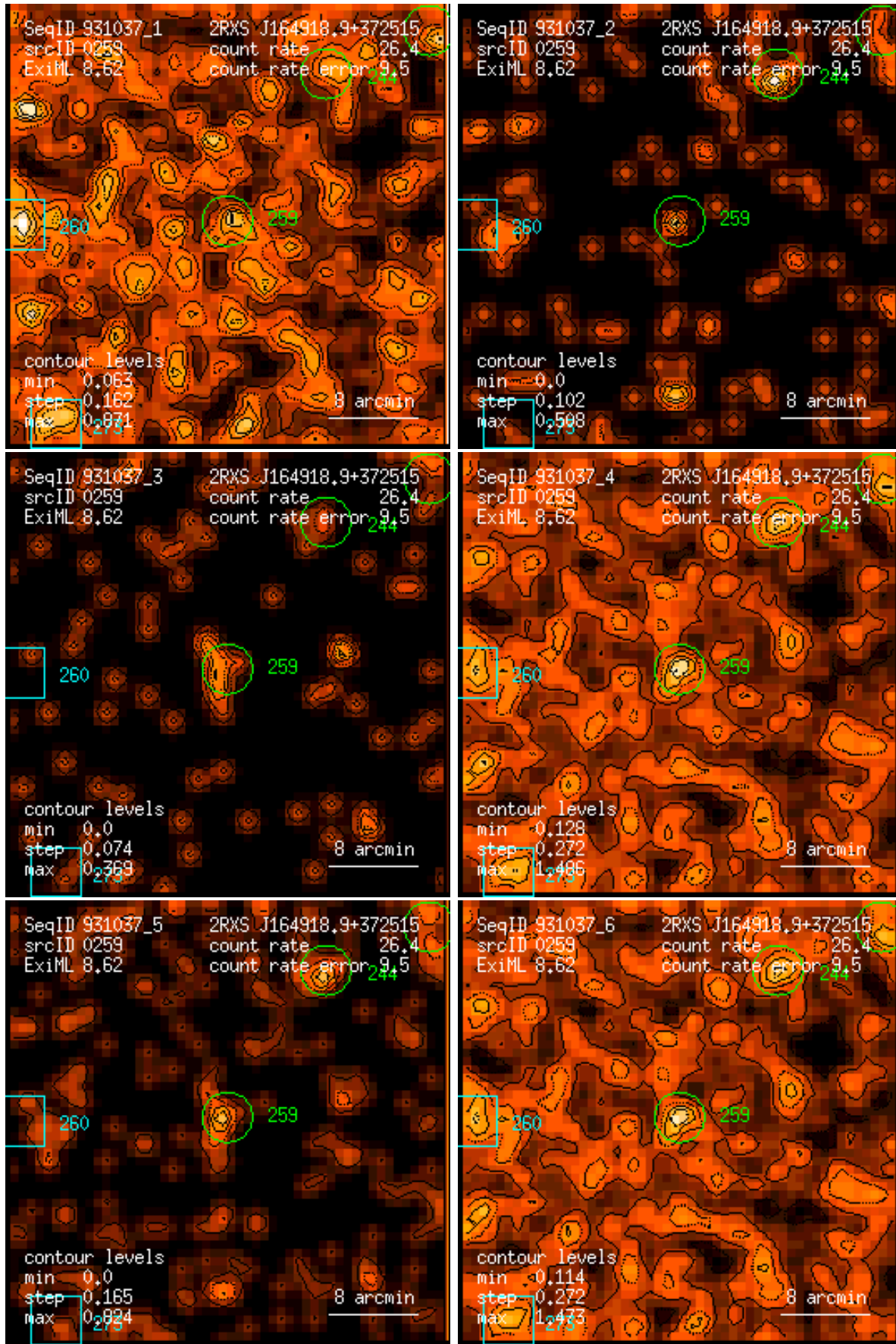
Figure 259: RASS 931037: detection 0259: band rate images, Gaussian filter: (1) PSPC channels 11 – 41, (2) 52 – 90, (3) 91 – 201, (4) 11 – 235, (5) 52 – 201, (6) 11 – 201. Broad band rates in counts/ks. Band rate contour levels in counts/ks/arcmin 2 .
