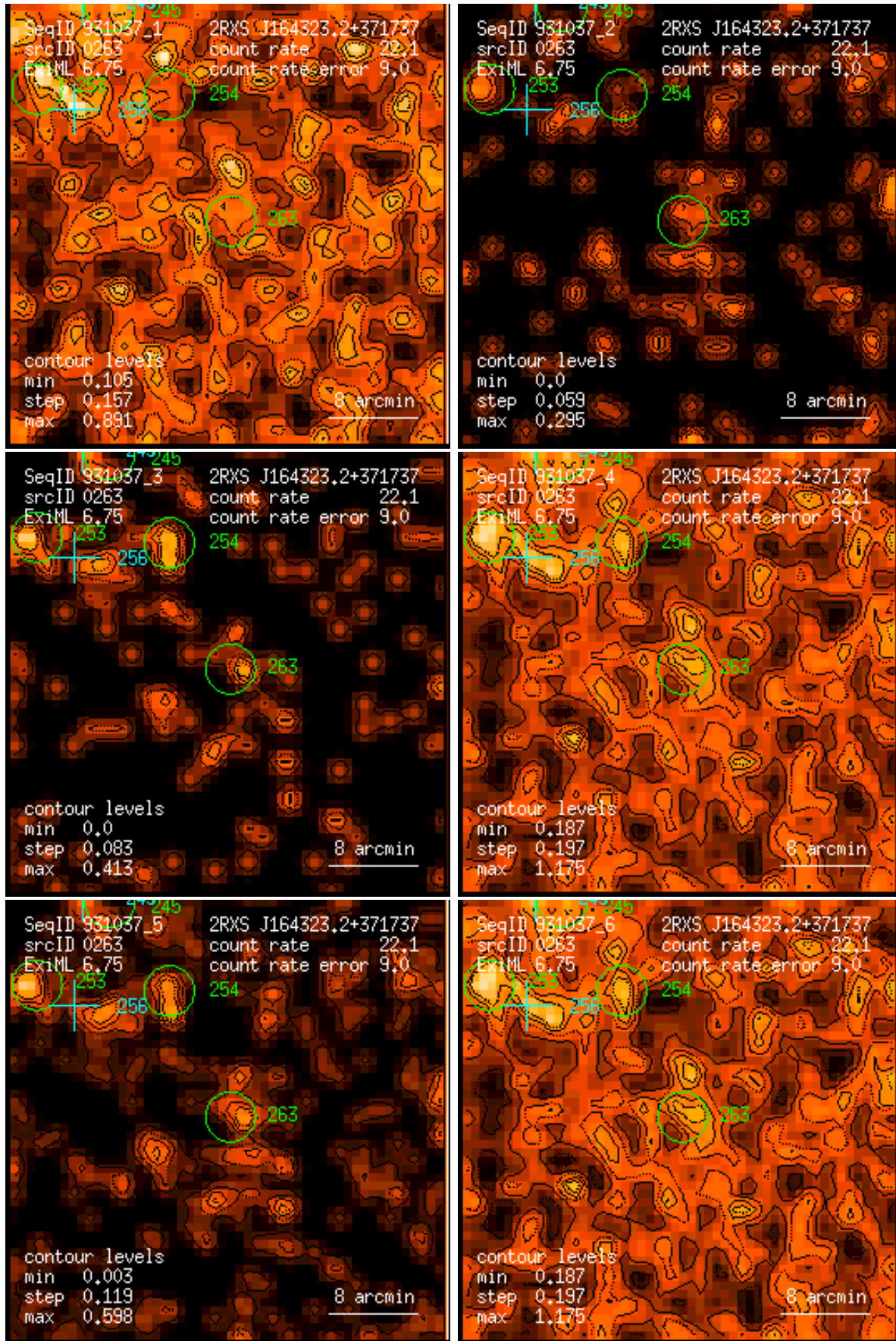
Figure 263: RASS 931037: detection 0263: band rate images, Gaussian filter: (1) PSPC channels 11 – 41, (2) 52 – 90, (3) 91 – 201, (4) 11 – 235, (5) 52 – 201, (6) 11 – 201. Broad band rates in counts/ks. Band rate contour levels in counts/ks/arcmin 2 .
