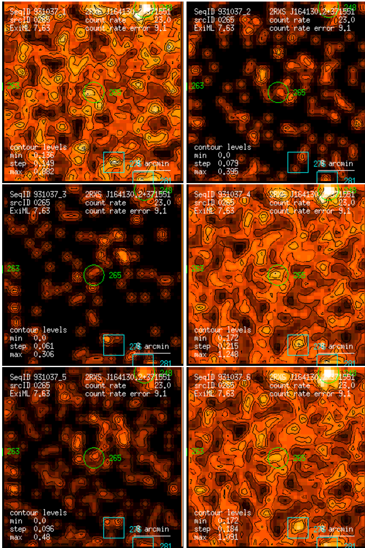
Figure 265: RASS 931037: detection 0265: band rate images, Gaussian filter: (1) PSPC channels 11 – 41, (2) 52 – 90, (3) 91 – 201, (4) 11 – 235, (5) 52 – 201, (6) 11 – 201. Broad band rates in counts/ks. Band rate contour levels in counts/ks/arcmin 2 .
