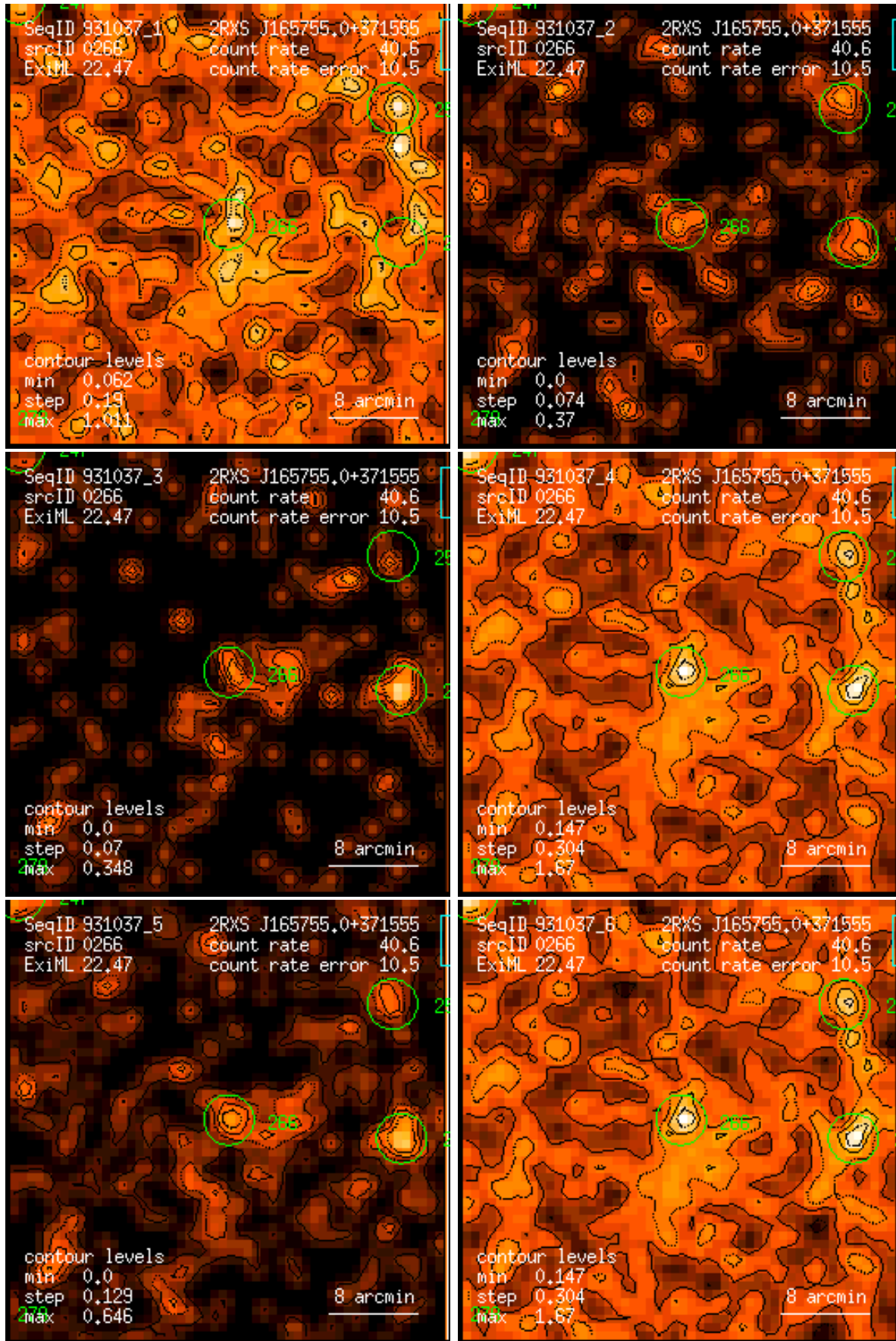
Figure 266: RASS 931037: detection 0266: band rate images, Gaussian filter: (1) PSPC channels 11 – 41, (2) 52 – 90, (3) 91 – 201, (4) 11 – 235, (5) 52 – 201, (6) 11 – 201. Broad band rates in counts/ks. Band rate contour levels in counts/ks/arcmin 2 .
