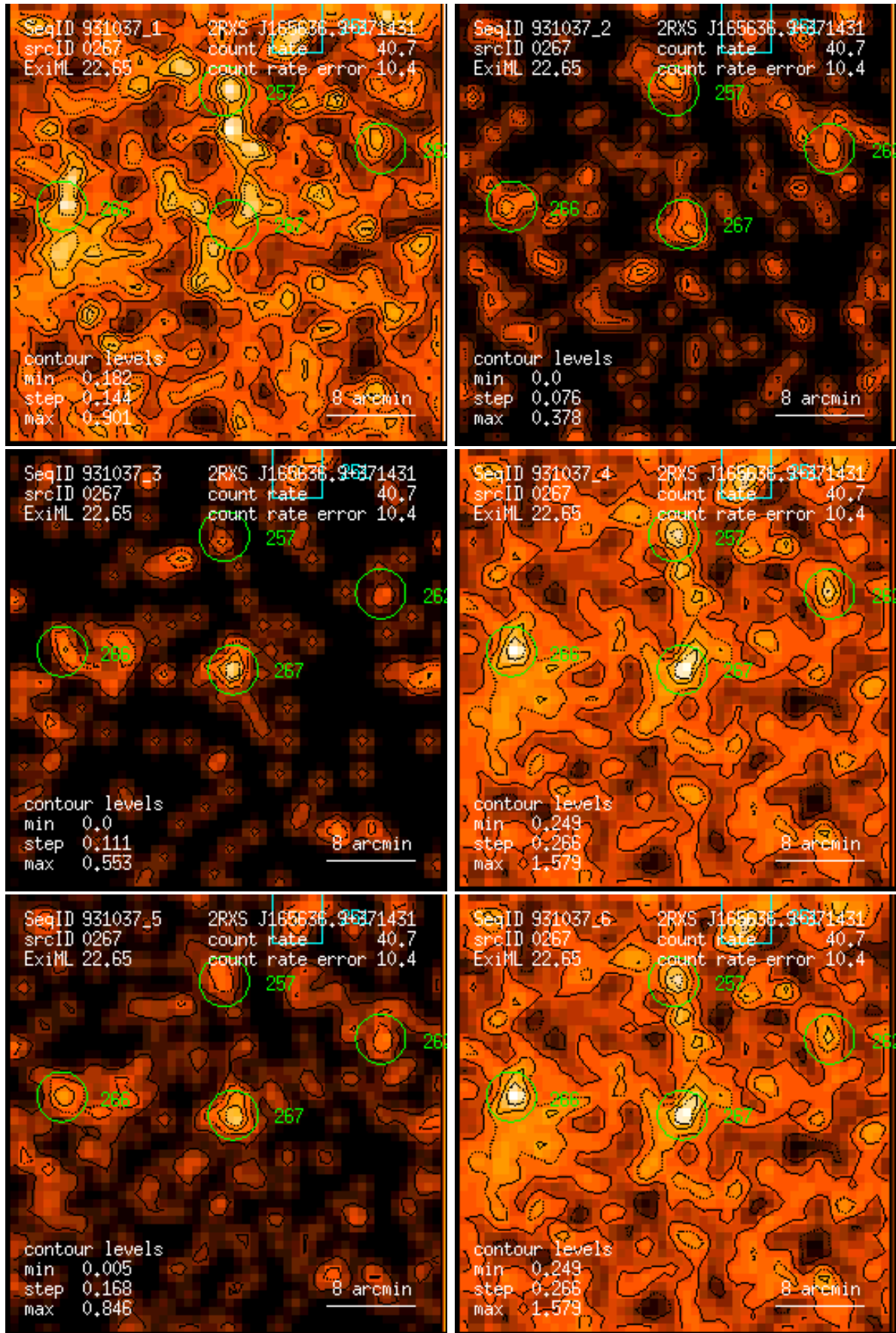
Figure 267: RASS 931037: detection 0267: band rate images, Gaussian filter: (1) PSPC channels 11 – 41, (2) 52 – 90, (3) 91 – 201, (4) 11 – 235, (5) 52 – 201, (6) 11 – 201. Broad band rates in counts/ks. Band rate contour levels in counts/ks/arcmin 2 .
