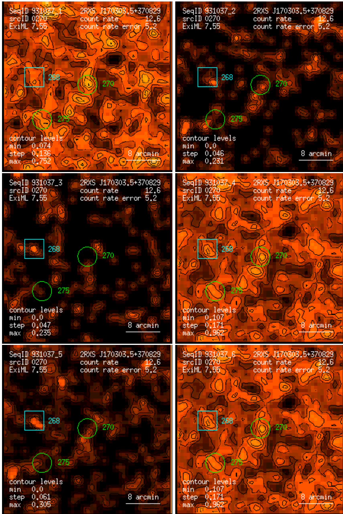
Figure 270: RASS 931037: detection 0270: band rate images, Gaussian filter: (1) PSPC channels 11 – 41, (2) 52 – 90, (3) 91 – 201, (4) 11 – 235, (5) 52 – 201, (6) 11 – 201. Broad band rates in counts/ks. Band rate contour levels in counts/ks/arcmin 2 .
