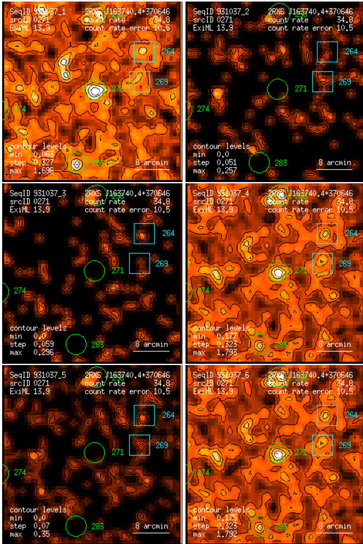
Figure 271: RASS 931037: detection 0271: band rate images, Gaussian filter: (1) PSPC channels 11 – 41, (2) 52 – 90, (3) 91 – 201, (4) 11 – 235, (5) 52 – 201, (6) 11 – 201. Broad band rates in counts/ks. Band rate contour levels in counts/ks/arcmin 2 .
