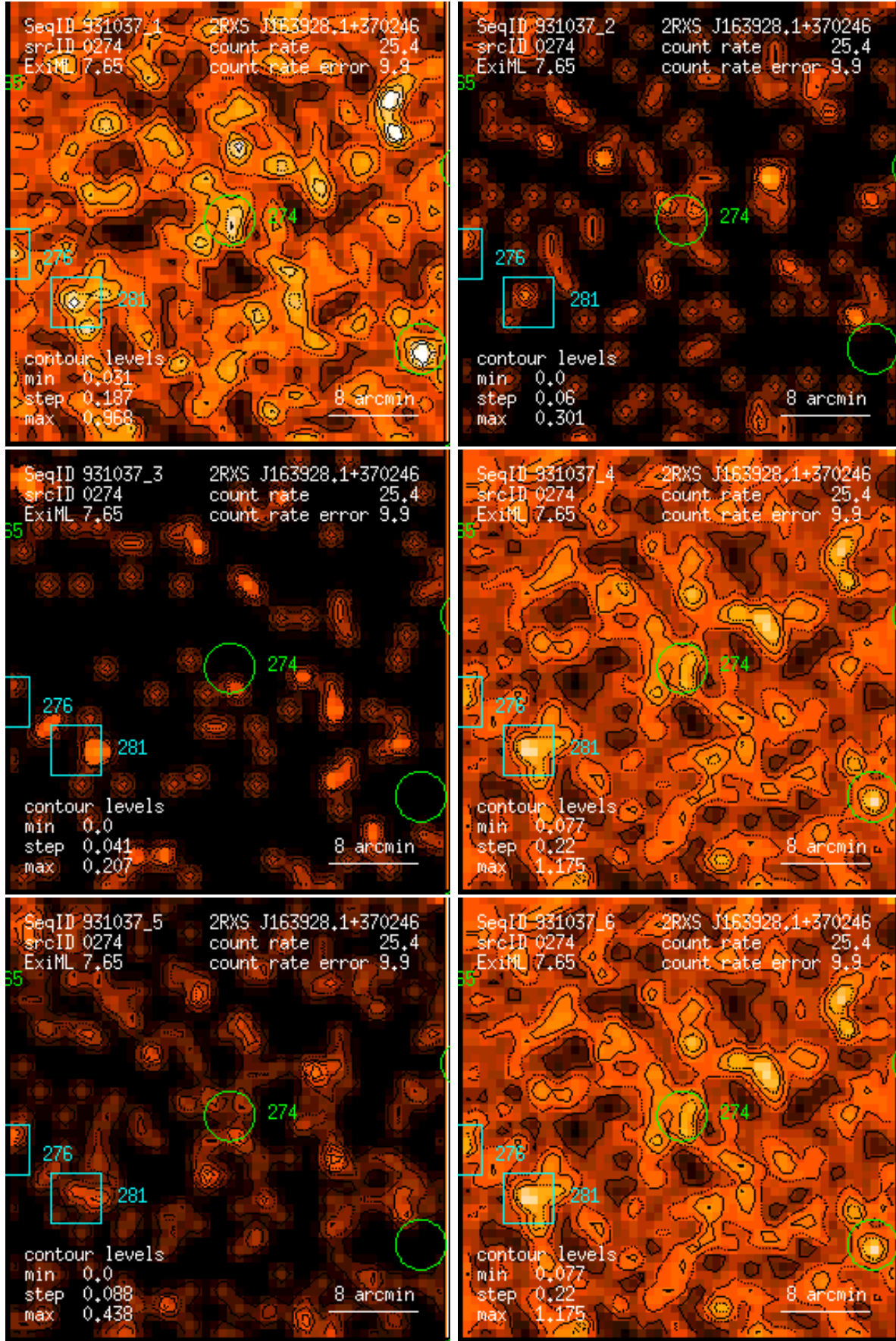
Figure 274: RASS 931037: detection 0274: band rate images, Gaussian filter: (1) PSPC channels 11 – 41, (2) 52 – 90, (3) 91 – 201, (4) 11 – 235, (5) 52 – 201, (6) 11 – 201. Broad band rates in counts/ks. Band rate contour levels in counts/ks/arcmin 2 .
