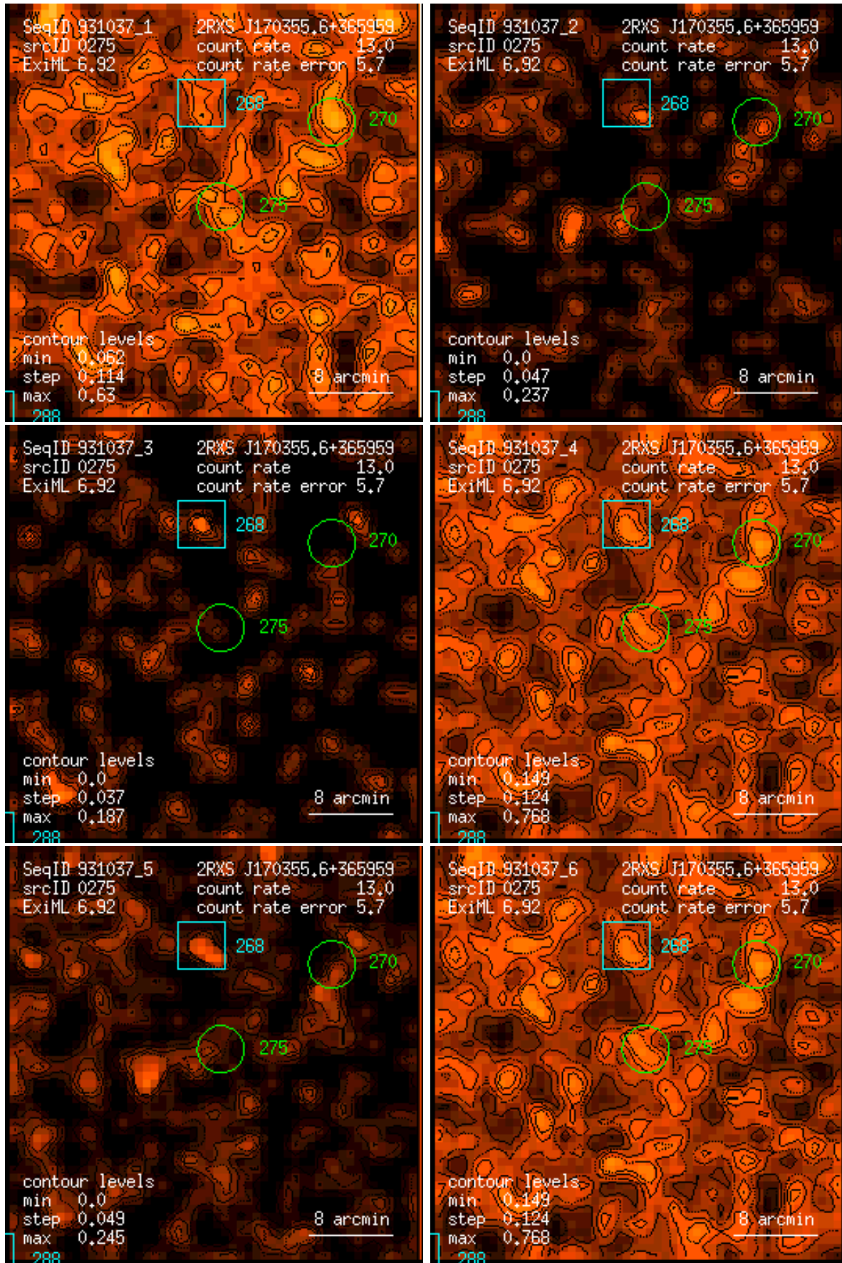
Figure 275: RASS 931037: detection 0275: band rate images, Gaussian filter: (1) PSPC channels 11 – 41, (2) 52 – 90, (3) 91 – 201, (4) 11 – 235, (5) 52 – 201, (6) 11 – 201. Broad band rates in counts/ks. Band rate contour levels in counts/ks/arcmin 2 .
