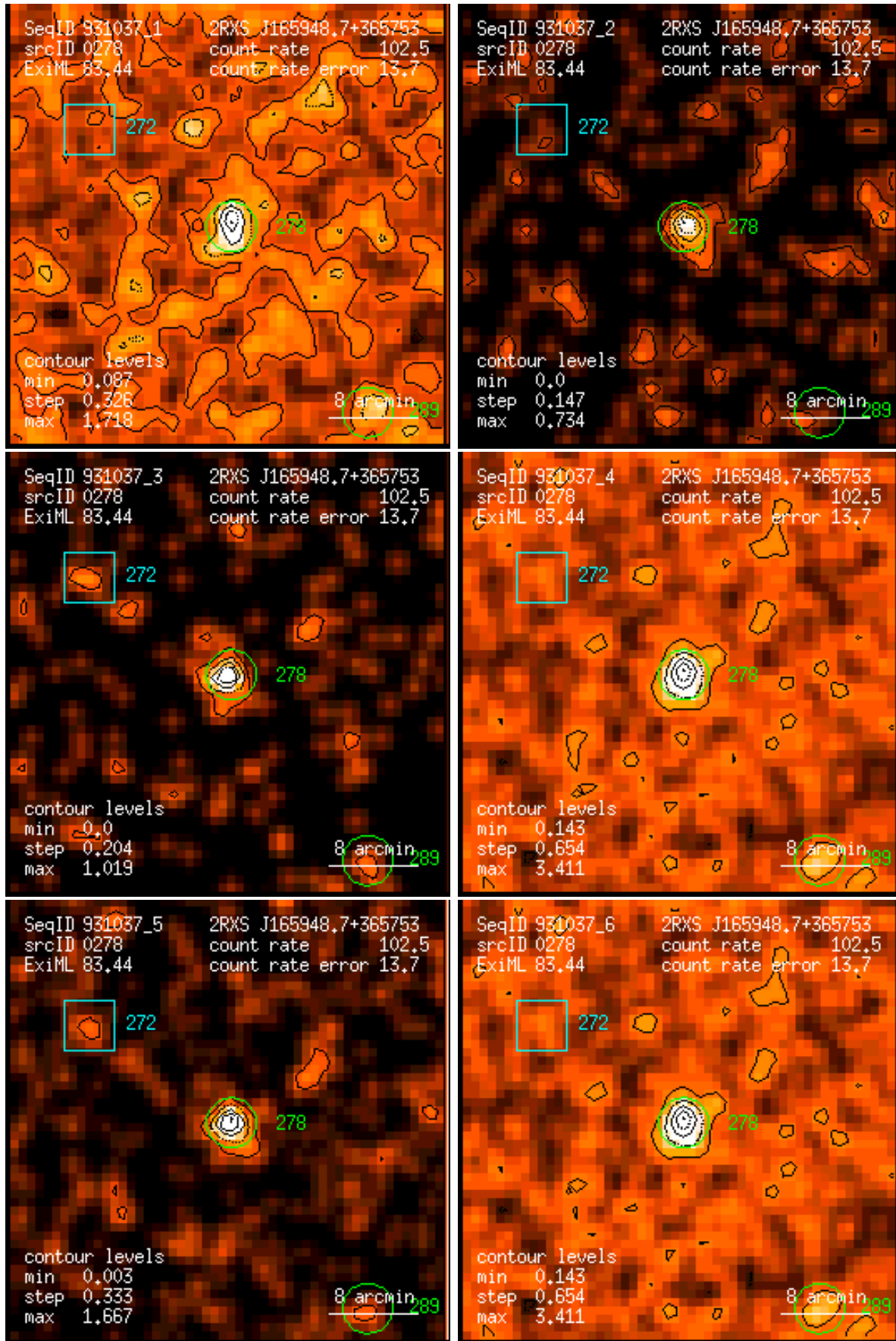
Figure 278: RASS 931037: detection 0278: band rate images, Gaussian filter: (1) PSPC channels 11 – 41, (2) 52 – 90, (3) 91 – 201, (4) 11 – 235, (5) 52 – 201, (6) 11 – 201. Broad band rates in counts/ks. Band rate contour levels in counts/ks/arcmin 2 .
