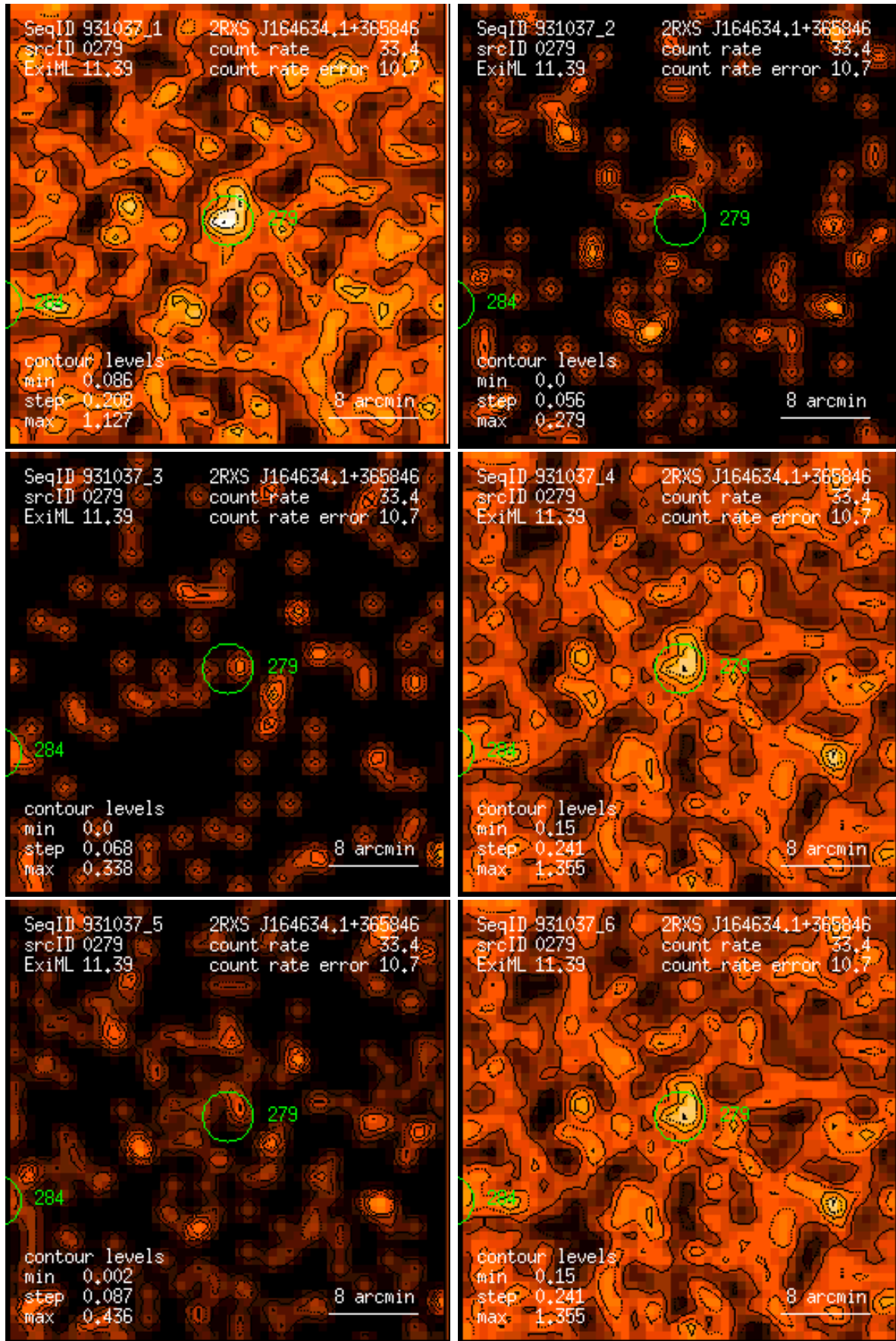
Figure 279: RASS 931037: detection 0279: band rate images, Gaussian filter: (1) PSPC channels 11 – 41, (2) 52 – 90, (3) 91 – 201, (4) 11 – 235, (5) 52 – 201, (6) 11 – 201. Broad band rates in counts/ks. Band rate contour levels in counts/ks/arcmin 2 .
