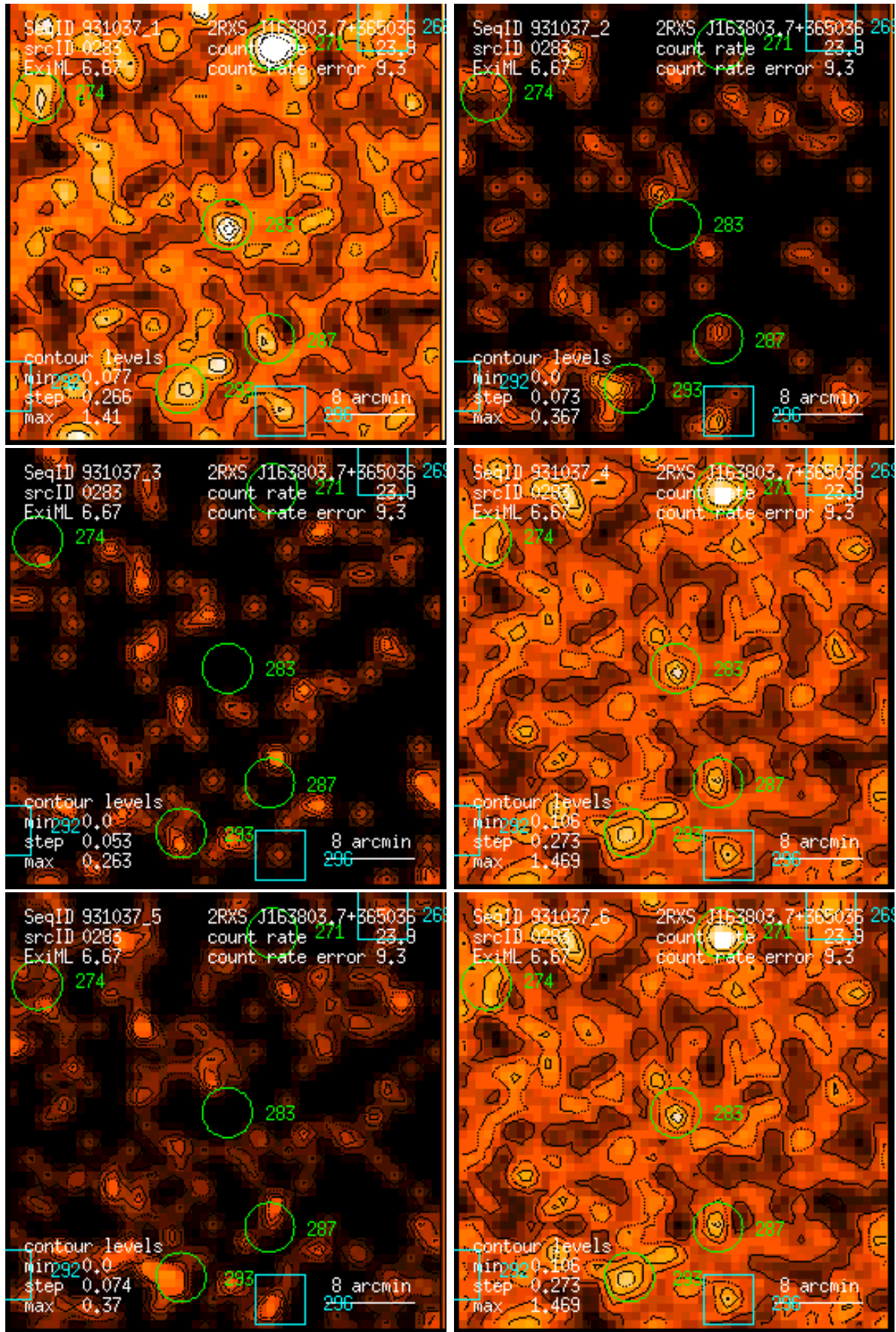
Figure 283: RASS 931037: detection 0283: band rate images, Gaussian filter: (1) PSPC channels 11 – 41, (2) 52 – 90, (3) 91 – 201, (4) 11 – 235, (5) 52 – 201, (6) 11 – 201. Broad band rates in counts/ks. Band rate contour levels in counts/ks/arcmin 2 .
