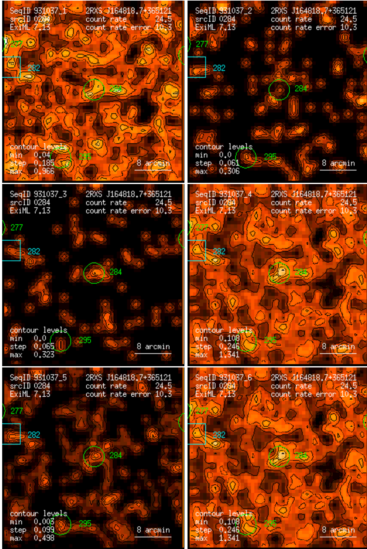
Figure 284: RASS 931037: detection 0284: band rate images, Gaussian filter: (1) PSPC channels 11 – 41, (2) 52 – 90, (3) 91 – 201, (4) 11 – 235, (5) 52 – 201, (6) 11 – 201. Broad band rates in counts/ks. Band rate contour levels in counts/ks/arcmin 2 .
