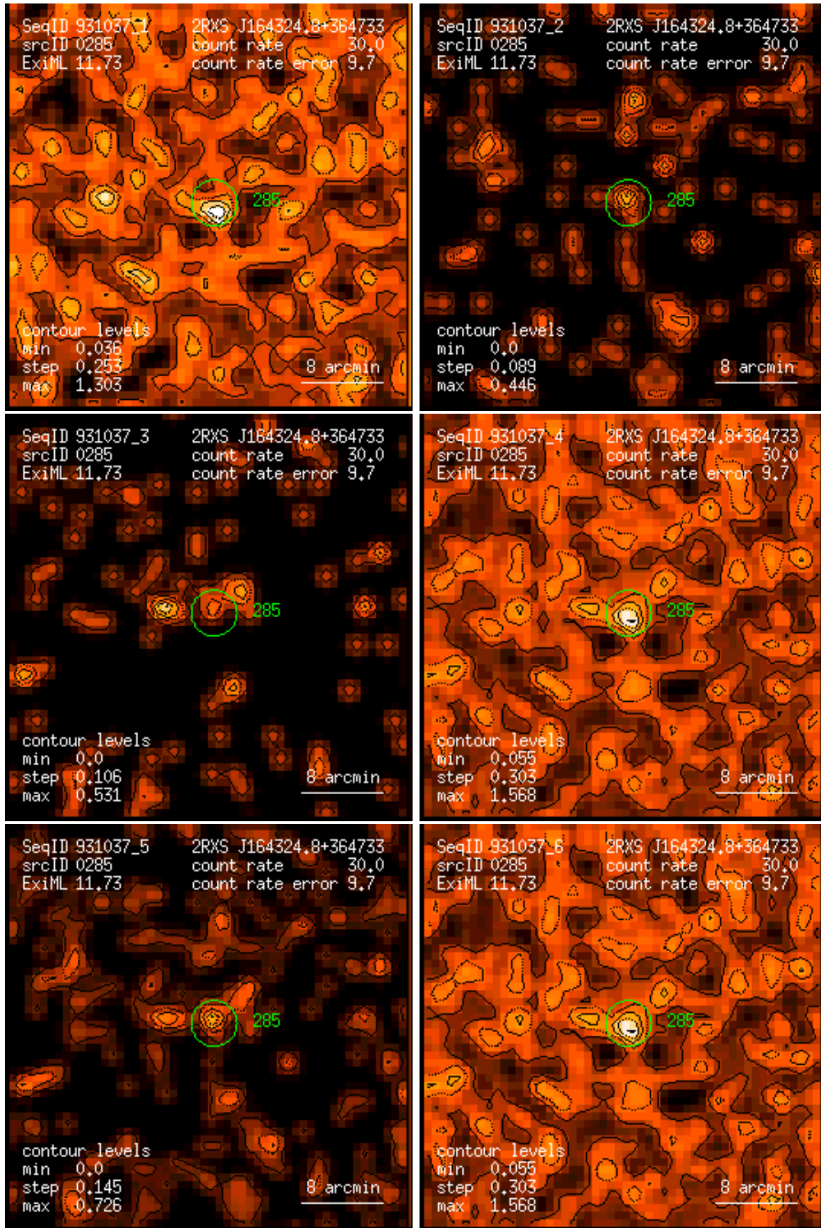
Figure 285: RASS 931037: detection 0285: band rate images, Gaussian filter: (1) PSPC channels 11 – 41, (2) 52 – 90, (3) 91 – 201, (4) 11 – 235, (5) 52 – 201, (6) 11 – 201. Broad band rates in counts/ks. Band rate contour levels in counts/ks/arcmin 2 .
