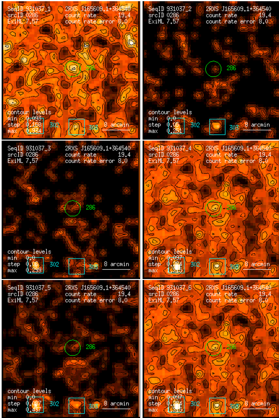
Figure 286: RASS 931037: detection 0286: band rate images, Gaussian filter: (1) PSPC channels 11 – 41, (2) 52 – 90, (3) 91 – 201, (4) 11 – 235, (5) 52 – 201, (6) 11 – 201. Broad band rates in counts/ks. Band rate contour levels in counts/ks/arcmin 2 .
