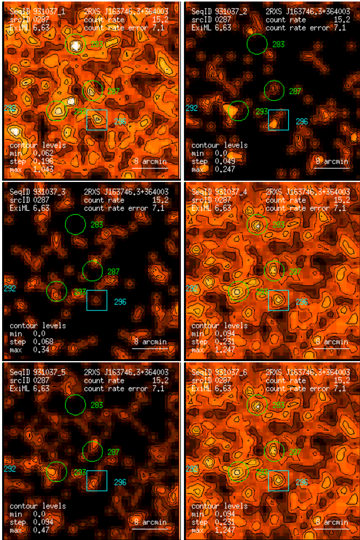
Figure 287: RASS 931037: detection 0287: band rate images, Gaussian filter: (1) PSPC channels 11 – 41, (2) 52 – 90, (3) 91 – 201, (4) 11 – 235, (5) 52 – 201, (6) 11 – 201. Broad band rates in counts/ks. Band rate contour levels in counts/ks/arcmin 2 .
