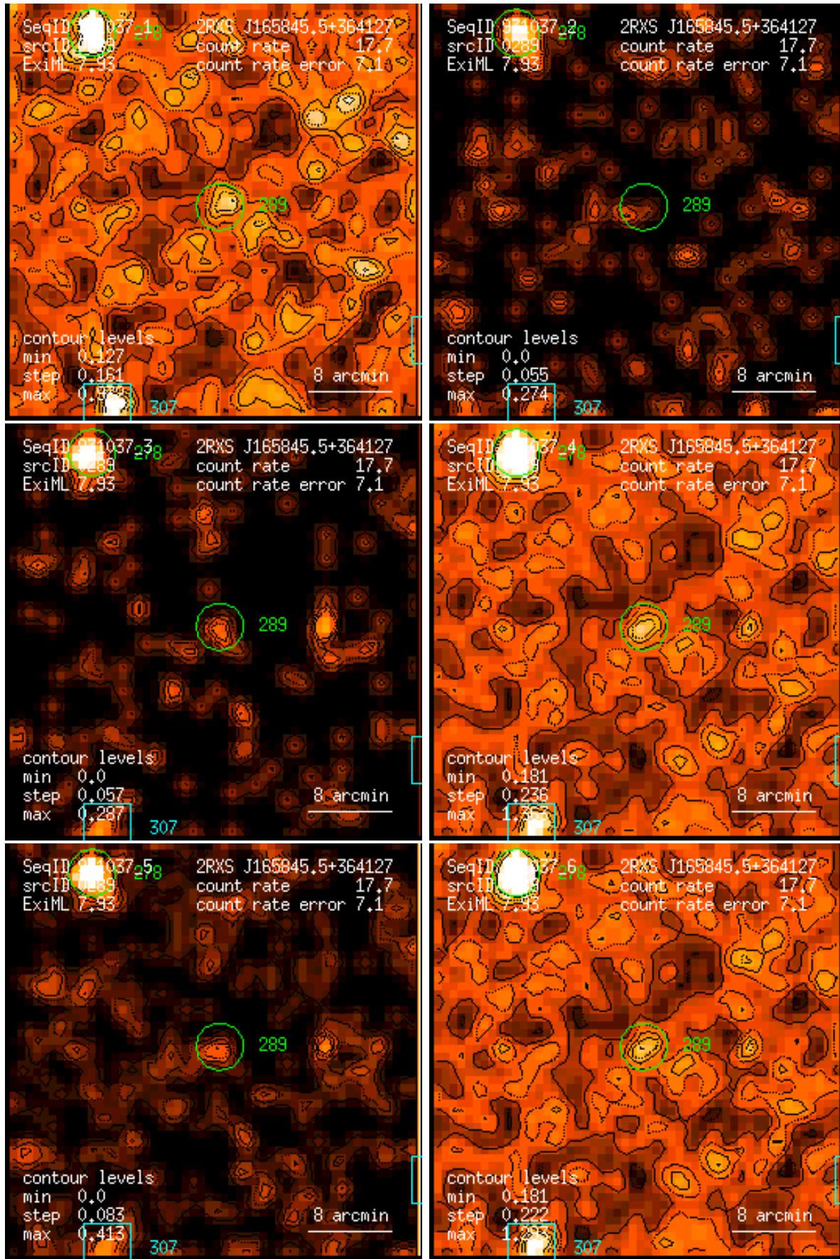
Figure 289: RASS 931037: detection 0289: band rate images, Gaussian filter: (1) PSPC channels 11 – 41, (2) 52 – 90, (3) 91 – 201, (4) 11 – 235, (5) 52 – 201, (6) 11 – 201. Broad band rates in counts/ks. Band rate contour levels in counts/ks/arcmin 2 .
