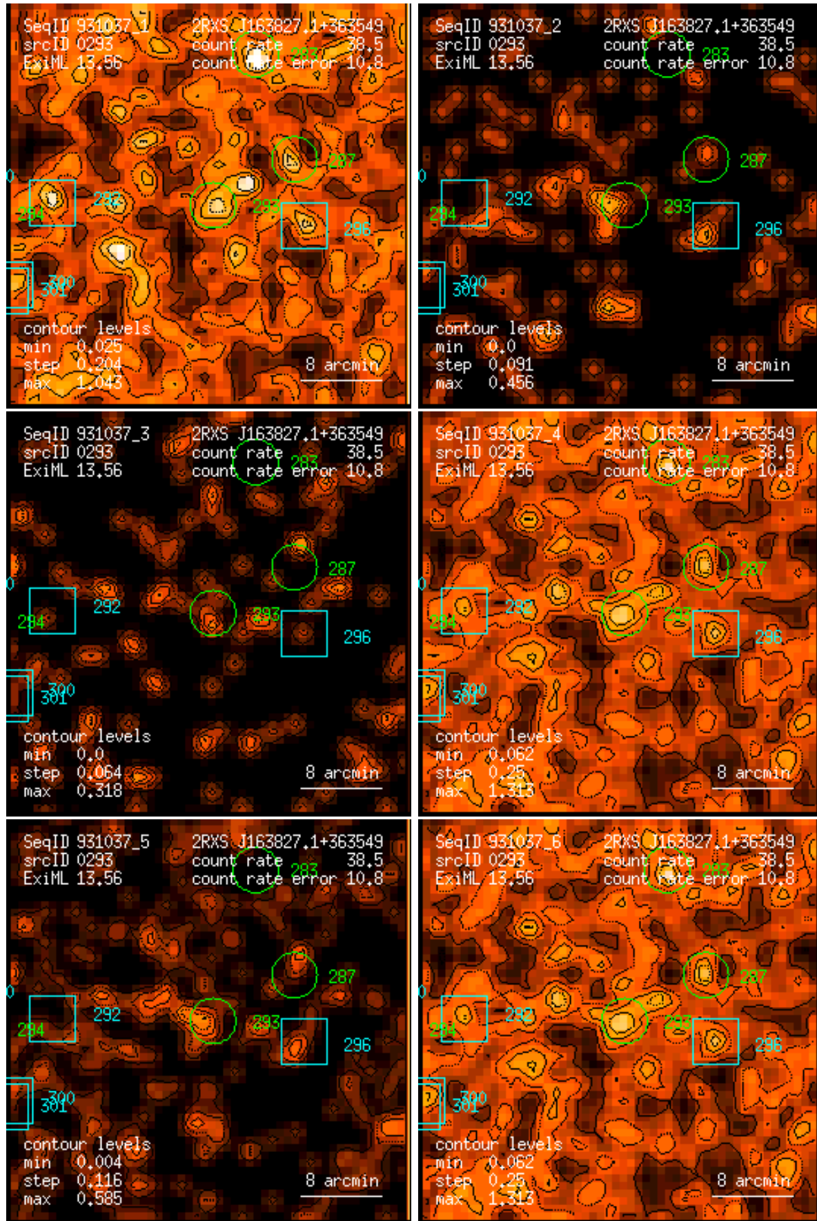
Figure 293: RASS 931037: detection 0293: band rate images, Gaussian filter: (1) PSPC channels 11 – 41, (2) 52 – 90, (3) 91 – 201, (4) 11 – 235, (5) 52 – 201, (6) 11 – 201. Broad band rates in counts/ks. Band rate contour levels in counts/ks/arcmin 2 .
