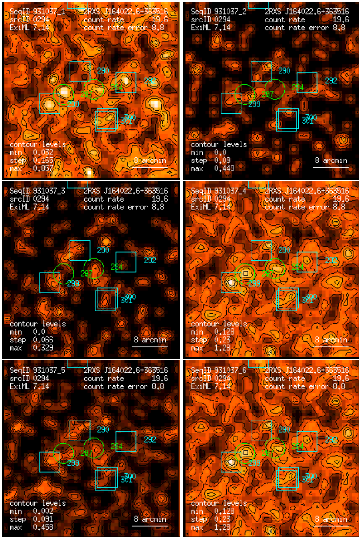
Figure 294: RASS 931037: detection 0294: band rate images, Gaussian filter: (1) PSPC channels 11 – 41, (2) 52 – 90, (3) 91 – 201, (4) 11 – 235, (5) 52 – 201, (6) 11 – 201. Broad band rates in counts/ks. Band rate contour levels in counts/ks/arcmin 2 .
