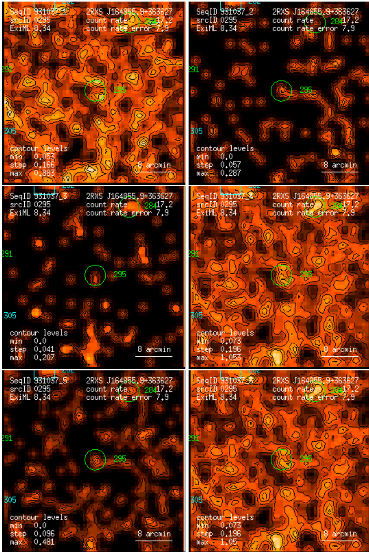
Figure 295: RASS 931037: detection 0295: band rate images, Gaussian filter: (1) PSPC channels 11 – 41, (2) 52 – 90, (3) 91 – 201, (4) 11 – 235, (5) 52 – 201, (6) 11 – 201. Broad band rates in counts/ks. Band rate contour levels in counts/ks/arcmin 2 .
