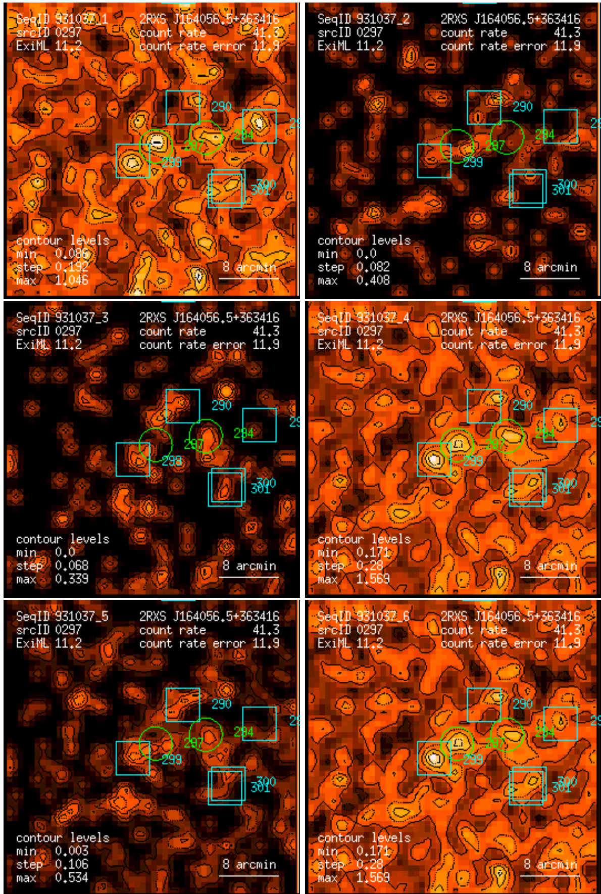
Figure 297: RASS 931037: detection 0297: band rate images, Gaussian filter: (1) PSPC channels 11 – 41, (2) 52 – 90, (3) 91 – 201, (4) 11 – 235, (5) 52 – 201, (6) 11 – 201. Broad band rates in counts/ks. Band rate contour levels in counts/ks/arcmin 2 .
