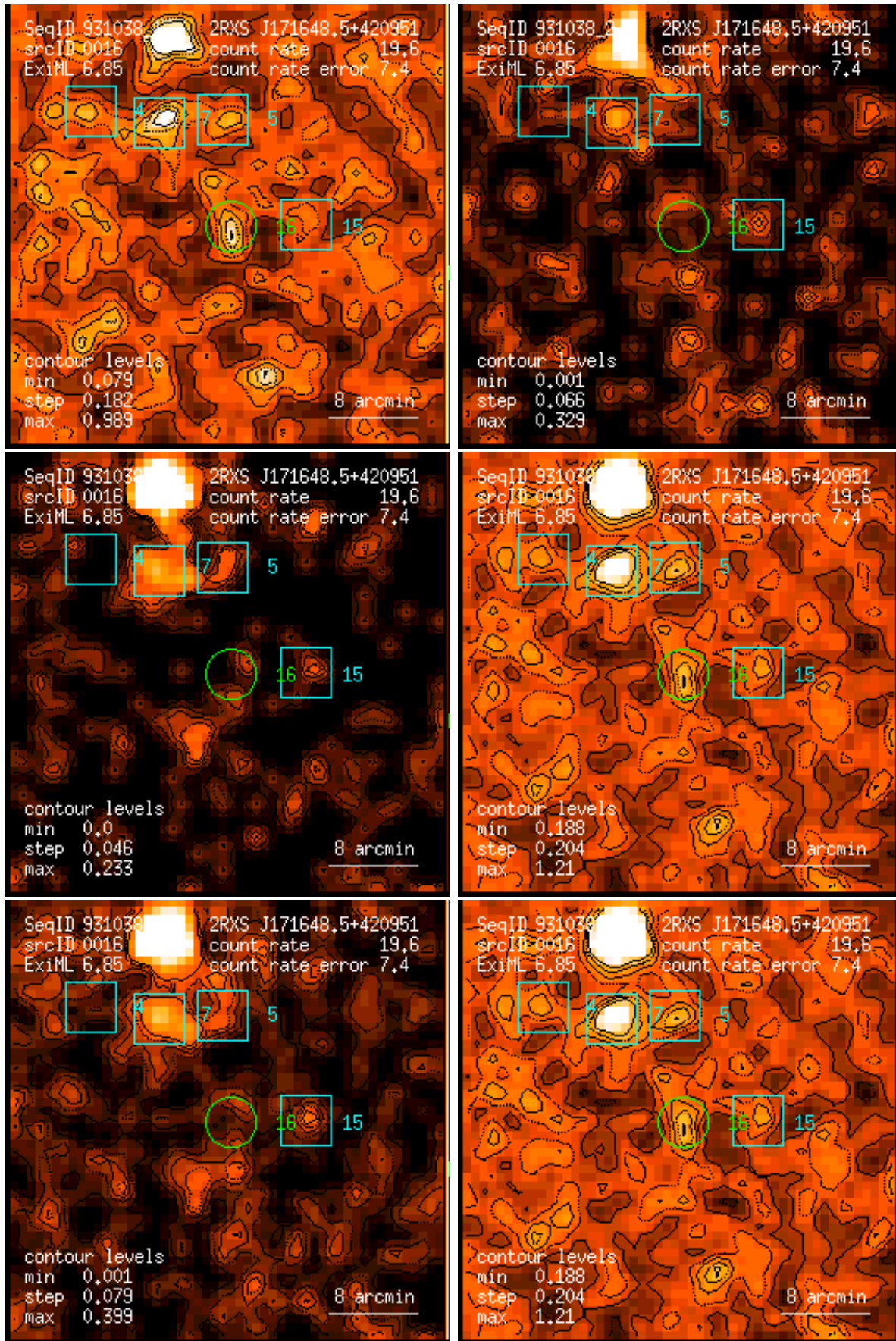
Figure 16: RASS 931038: detection 0016: band rate images, Gaussian filter: (1) PSPC channels 11 – 41, (2) 52 – 90, (3) 91 – 201, (4) 11 – 235, (5) 52 – 201, (6) 11 – 201. Broad band rates in counts/ks. Band rate contour levels in counts/ks/arcmin 2 .
