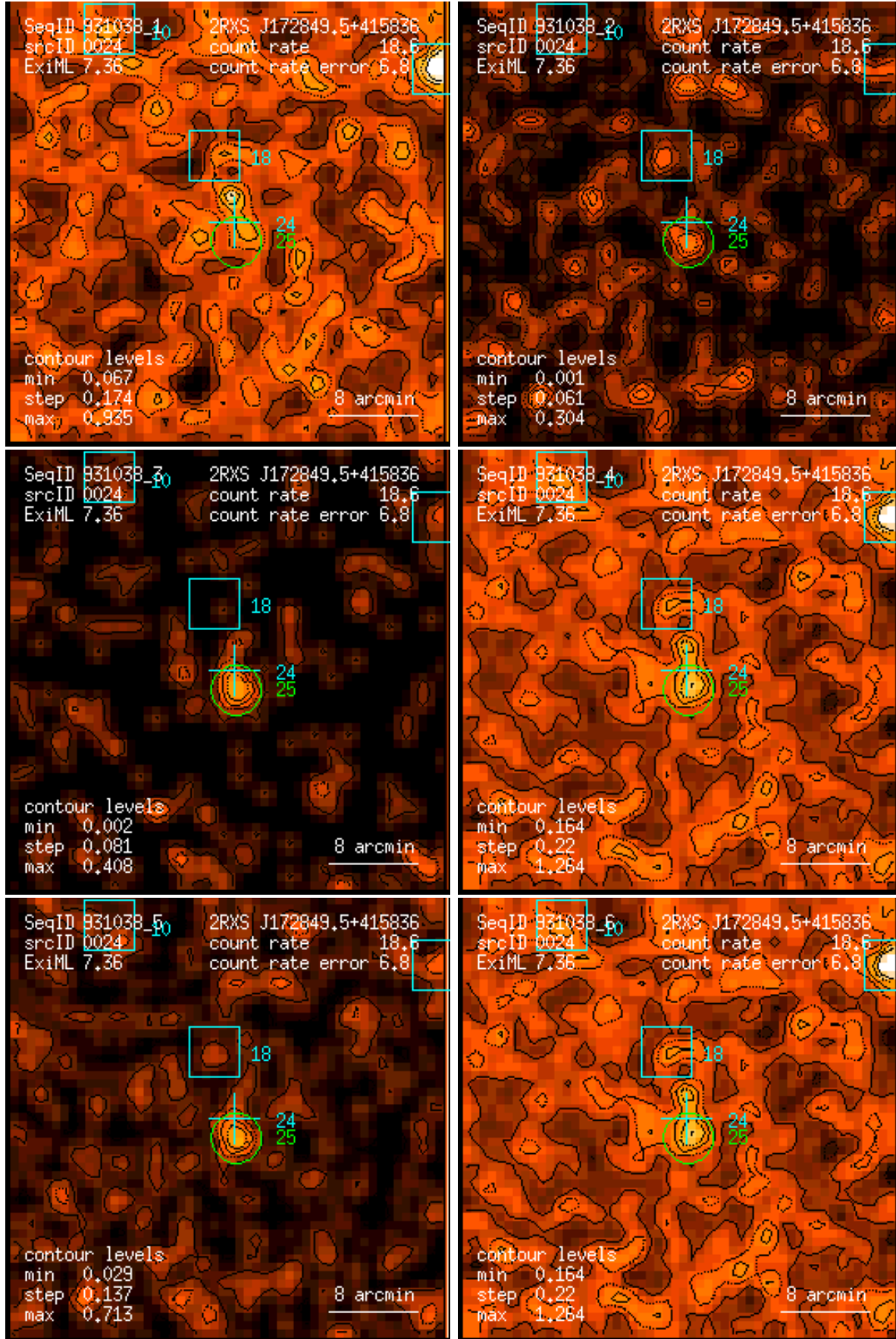
Figure 24: RASS 931038: detection 0024: band rate images, Gaussian filter: (1) PSPC channels 11 – 41, (2) 52 – 90, (3) 91 – 201, (4) 11 – 235, (5) 52 – 201, (6) 11 – 201. Broad band rates in counts/ks. Band rate contour levels in counts/ks/arcmin 2 .
