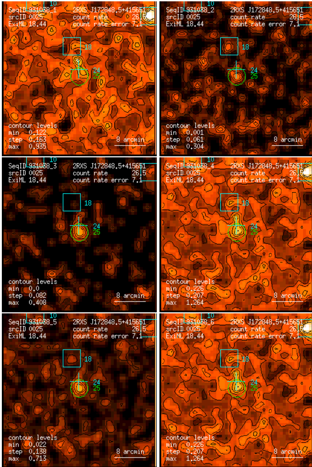
Figure 25: RASS 931038: detection 0025: band rate images, Gaussian filter: (1) PSPC channels 11 – 41, (2) 52 – 90, (3) 91 – 201, (4) 11 – 235, (5) 52 – 201, (6) 11 – 201. Broad band rates in counts/ks. Band rate contour levels in counts/ks/arcmin 2 .
