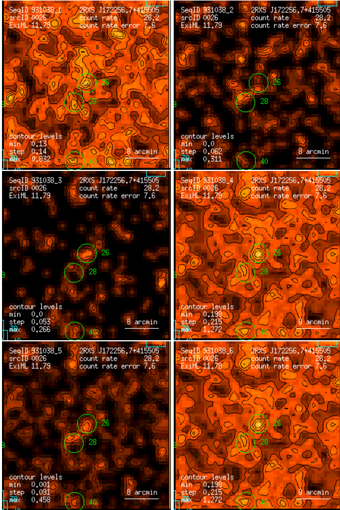
Figure 26: RASS 931038: detection 0026: band rate images, Gaussian filter: (1) PSPC channels 11 – 41, (2) 52 – 90, (3) 91 – 201, (4) 11 – 235, (5) 52 – 201, (6) 11 – 201. Broad band rates in counts/ks. Band rate contour levels in counts/ks/arcmin 2 .
