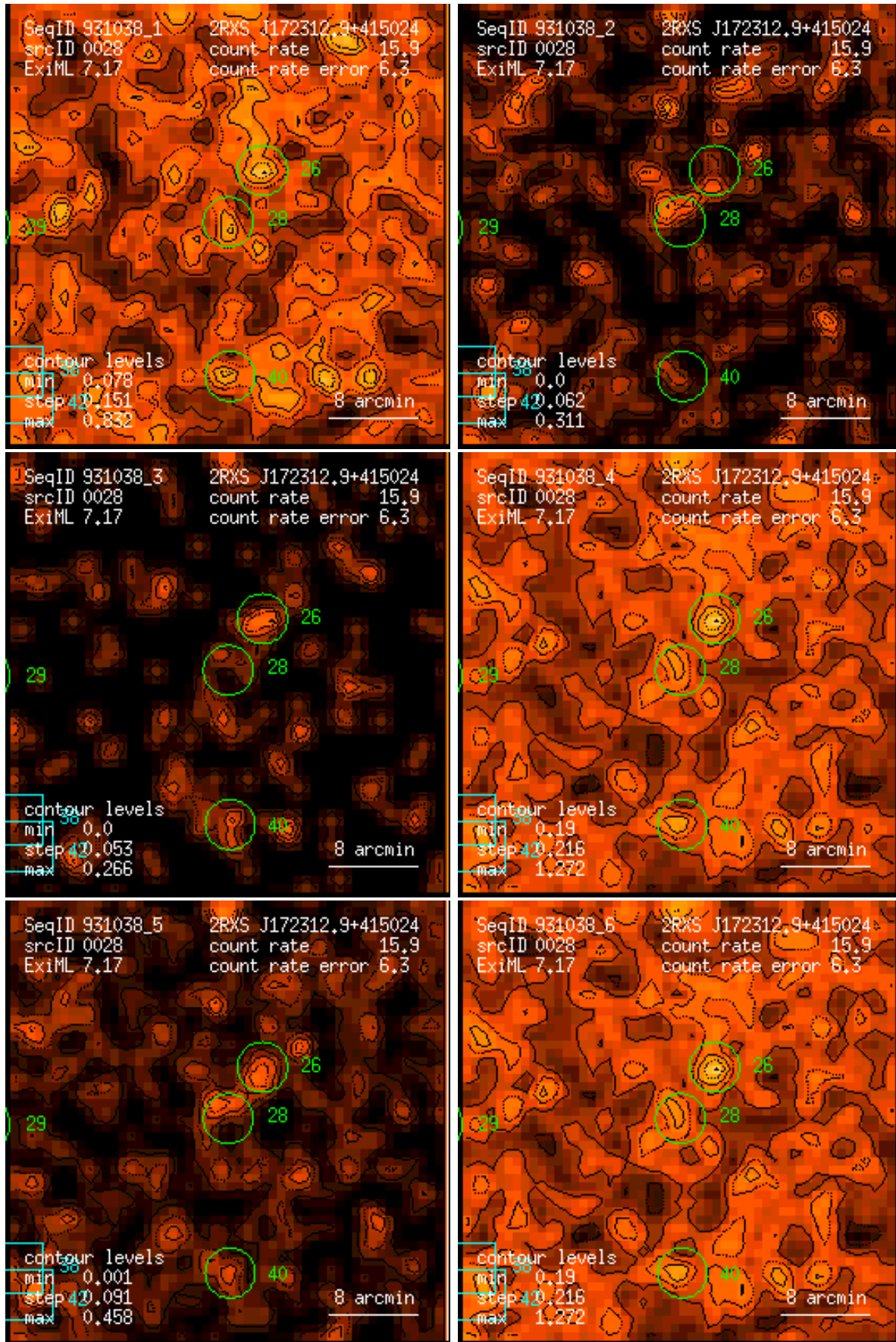
Figure 28: RASS 931038: detection 0028: band rate images, Gaussian filter: (1) PSPC channels 11 – 41, (2) 52 – 90, (3) 91 – 201, (4) 11 – 235, (5) 52 – 201, (6) 11 – 201. Broad band rates in counts/ks. Band rate contour levels in counts/ks/arcmin 2 .
