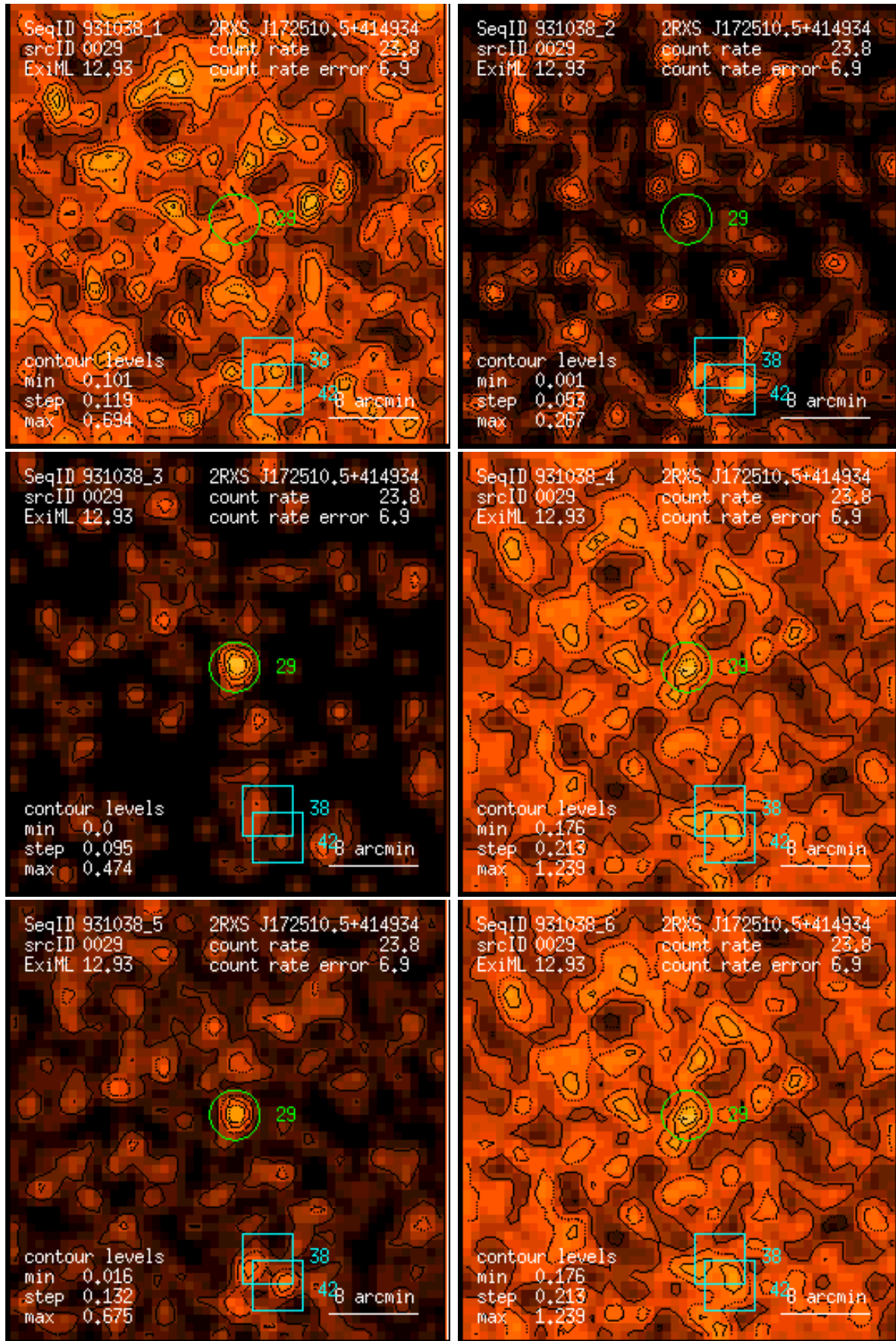
Figure 29: RASS 931038: detection 0029: band rate images, Gaussian filter: (1) PSPC channels 11 – 41, (2) 52 – 90, (3) 91 – 201, (4) 11 – 235, (5) 52 – 201, (6) 11 – 201. Broad band rates in counts/ks. Band rate contour levels in counts/ks/arcmin 2 .
