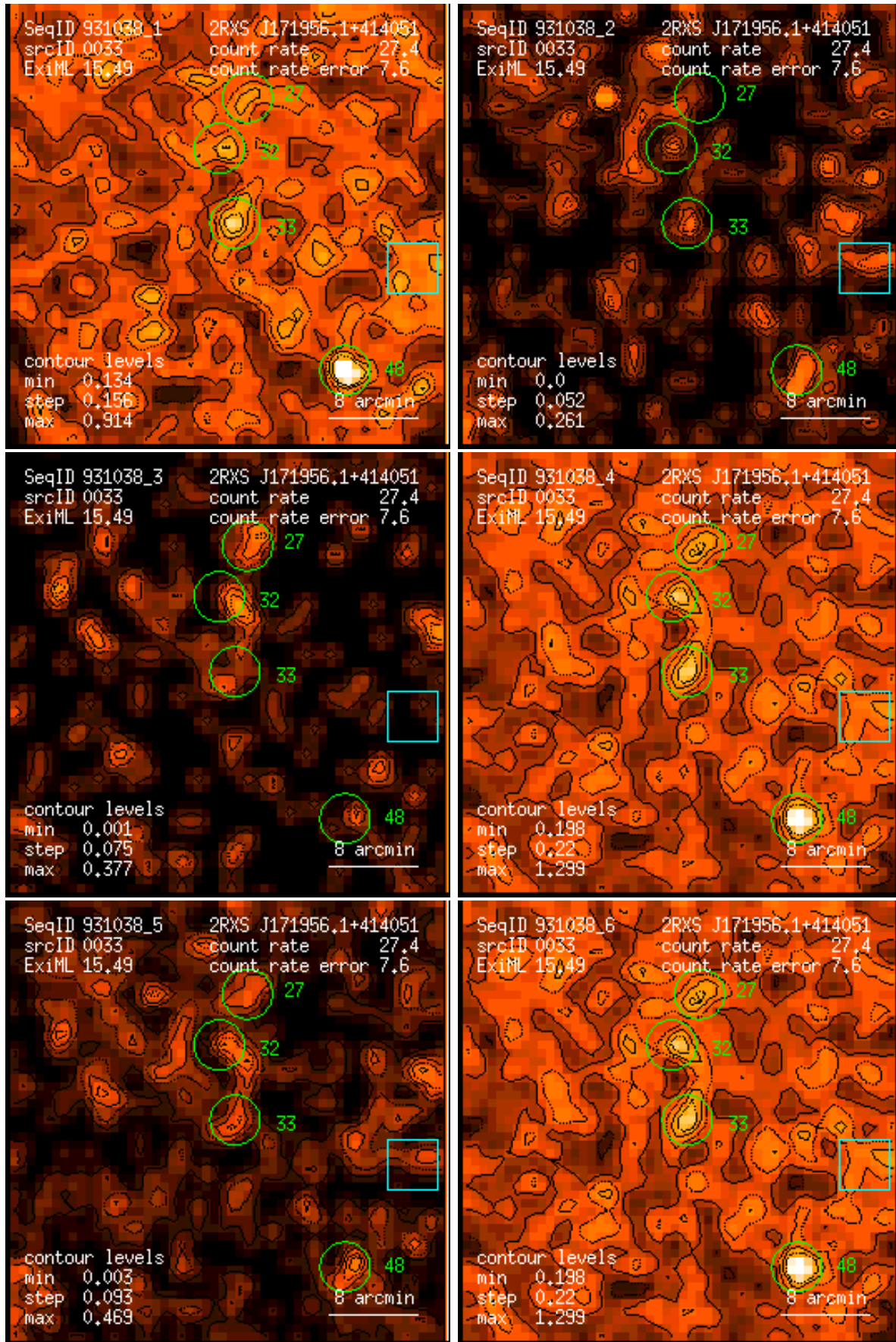
Figure 33: RASS 931038: detection 0033: band rate images, Gaussian filter: (1) PSPC channels 11 – 41, (2) 52 – 90, (3) 91 – 201, (4) 11 – 235, (5) 52 – 201, (6) 11 – 201. Broad band rates in counts/ks. Band rate contour levels in counts/ks/arcmin 2 .
